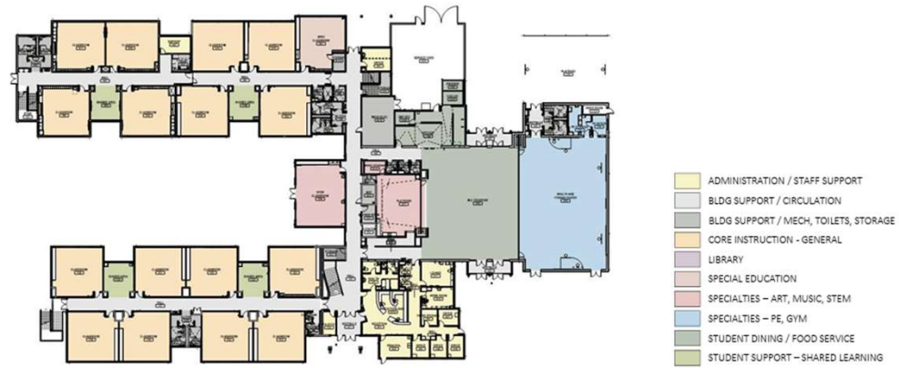
OVERALL LEVEL 1 FLOOR PLAN
