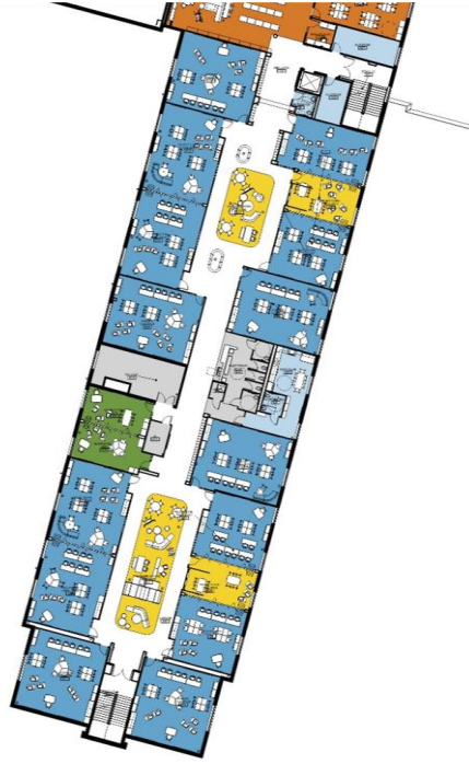
Level 02
