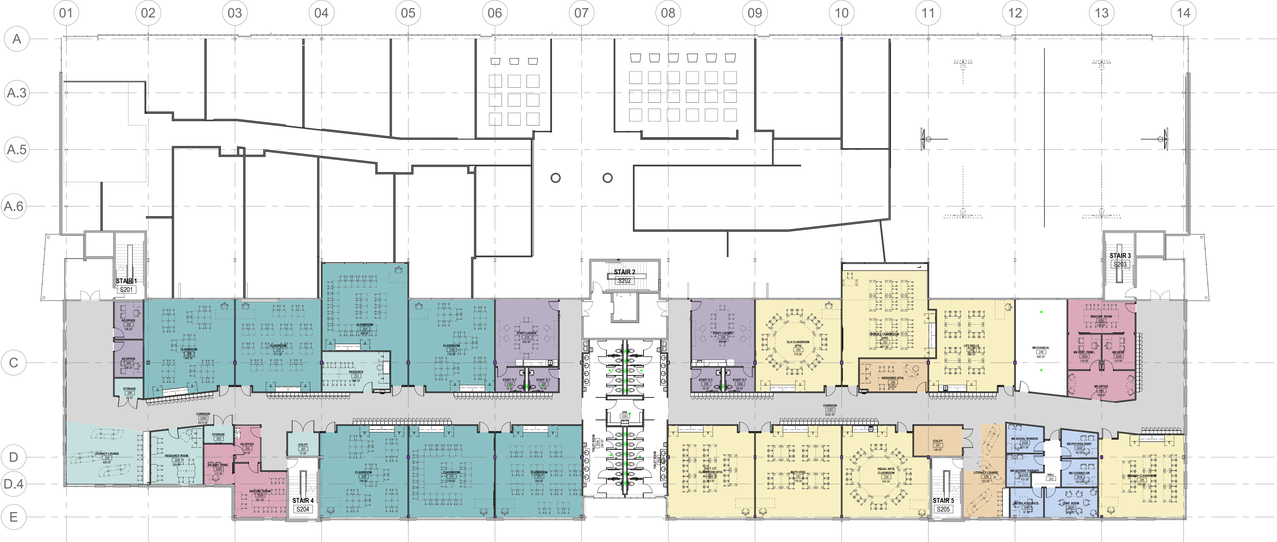
2 SECOND FLOOR PLAN A100 1/16" = 1'-0"
