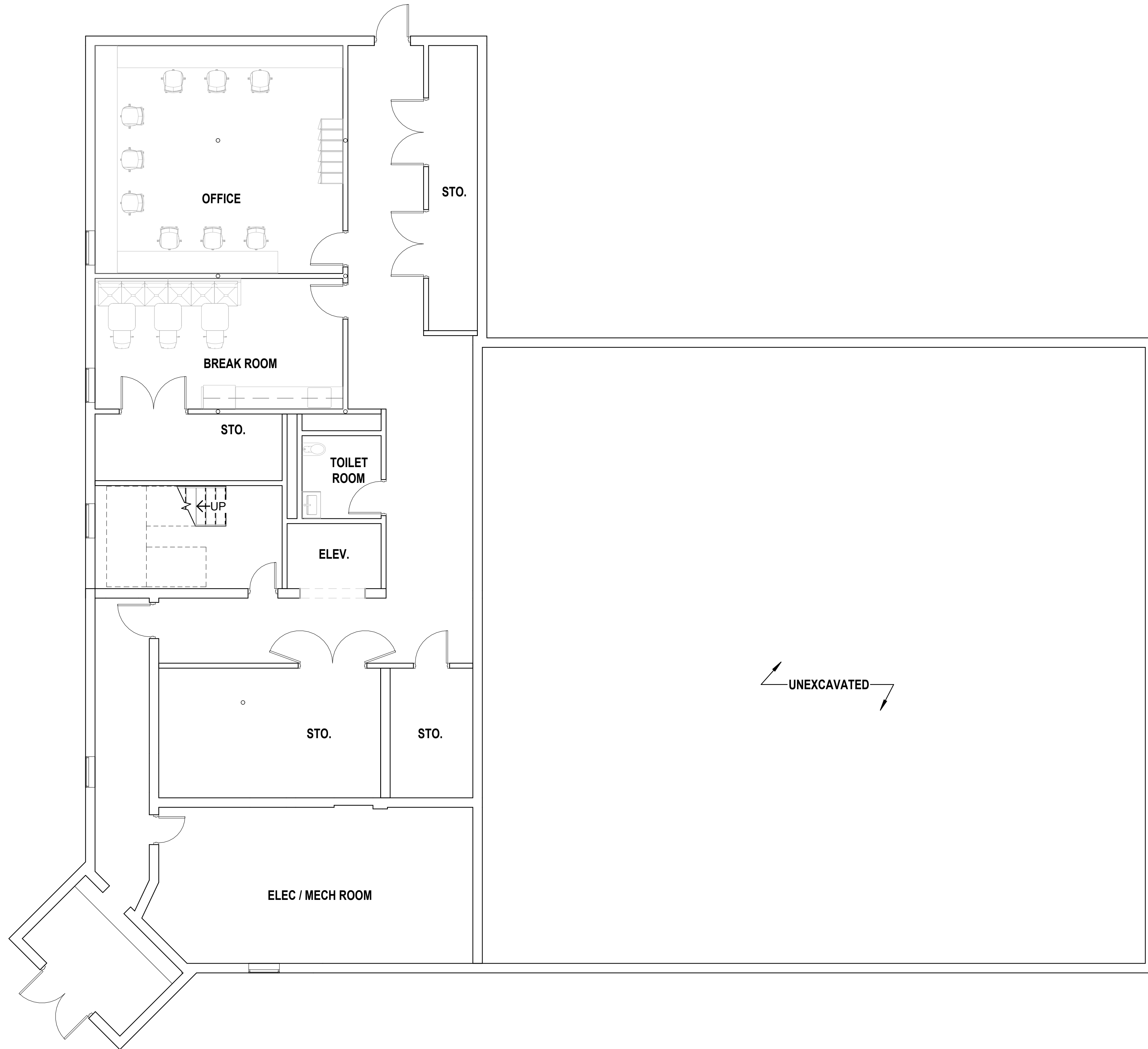
Proposed Lower Level Floor Plan
