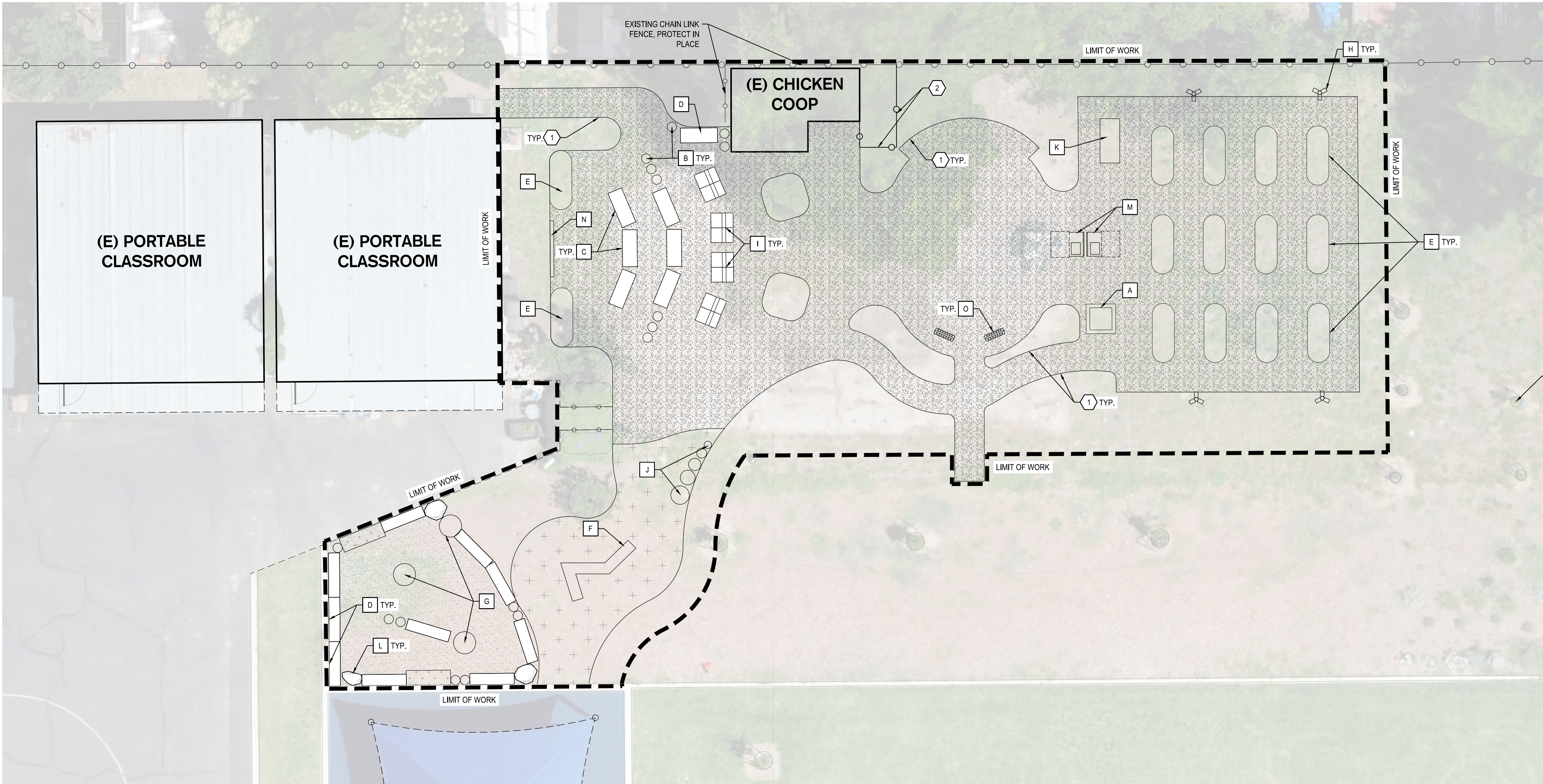
AMENITIES PLAN
