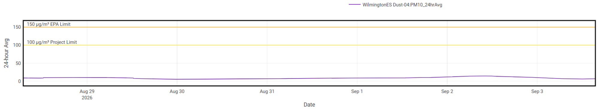
WilmingtonES Dust-04 PM10 ( \mu\text{g}/\text{m}^3 )
