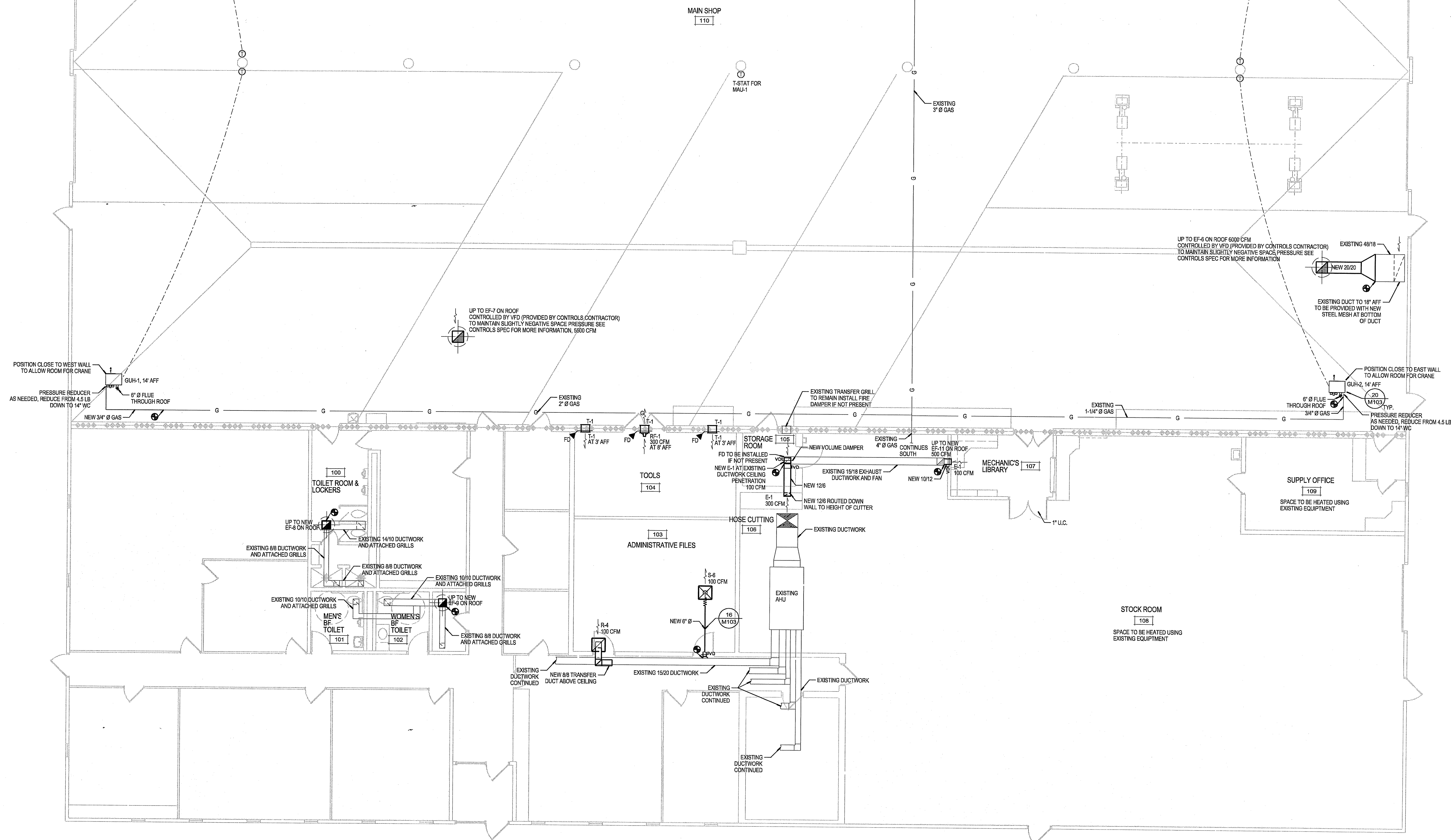
ENLARGED HVAC PLAN - SOUTH SCALE: 1/8"=1'-0"
