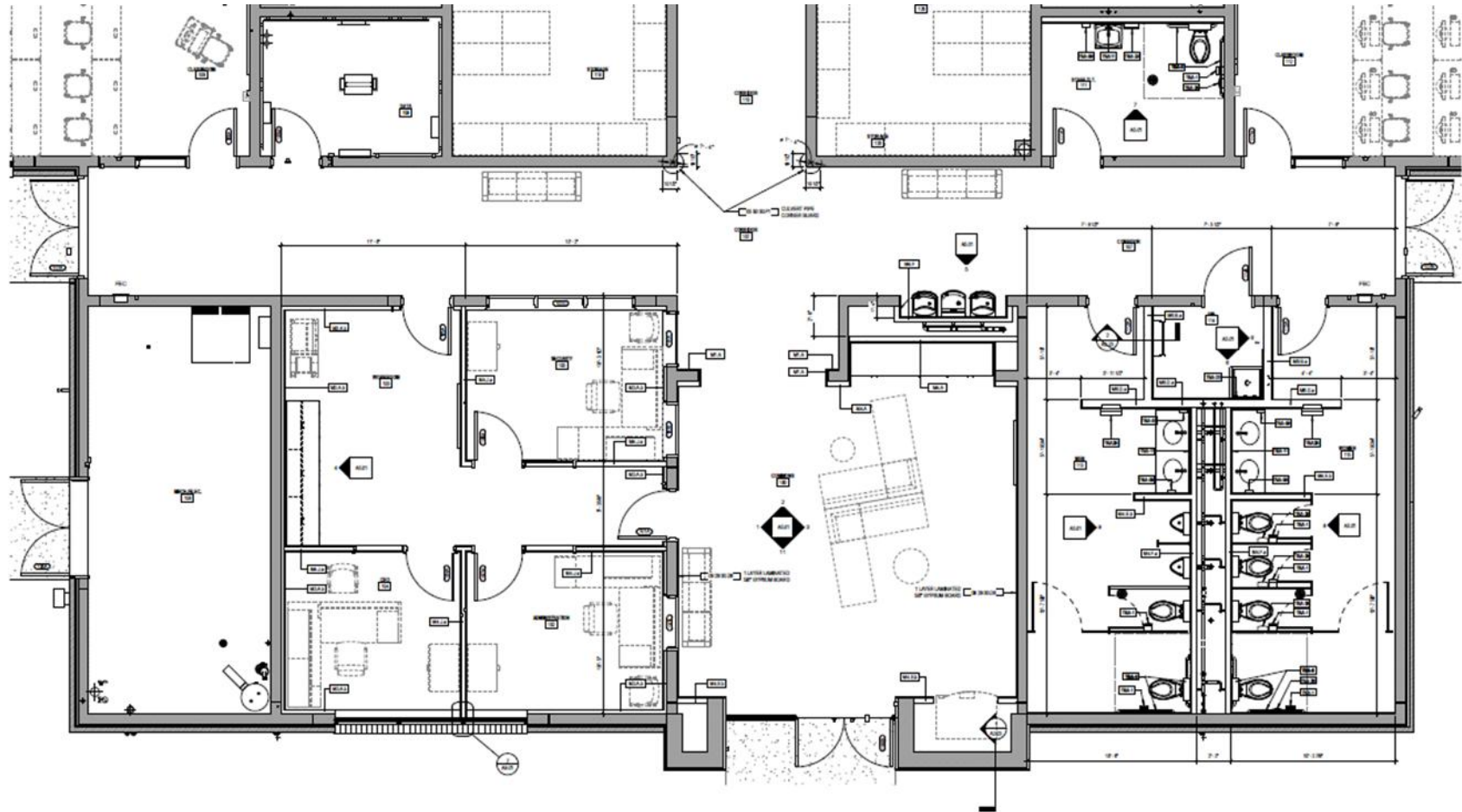
Sample Administrative, Lobby, Mechanical Room and Restroom Areas Shown (Instructional Areas Shown on Previous Page)
