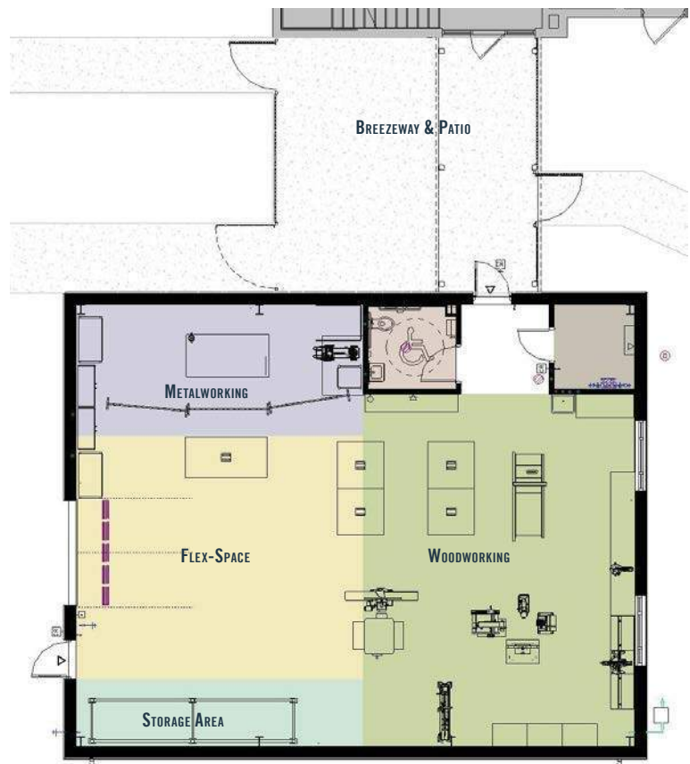
▲ Floor Plan
