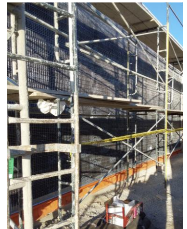
Lath at kitchen expansion exterior complete. Stucco to follow.
