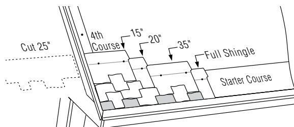
Figure 14-15: Fourth Course.
