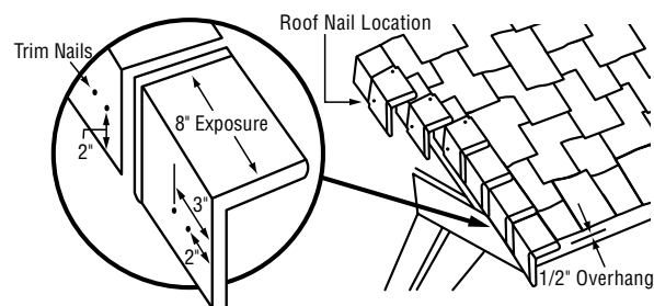
Figure 14-18: Mountain Ridge Rake edge application.
