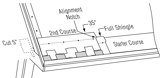
Figure 14-13: Second Course.
