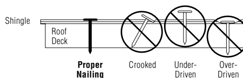
Figure 14-5: Proper and improper nailing.
