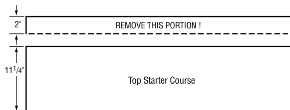
Figure 14-10: Presidential Starter (top starter course.)
