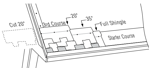
Figure 14-14: Third Course.
