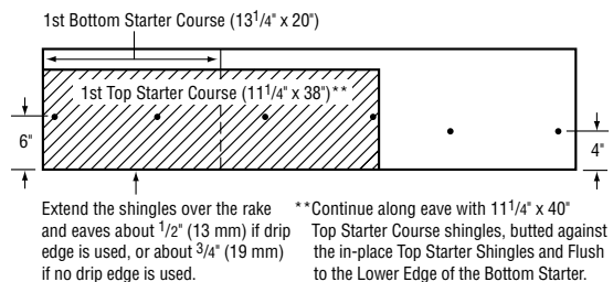
Figure 14-11: Use two (2) overlapping layers of CertainTeed's "Presidential Starter."
