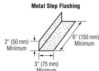
Figure 14-23: Metal step flashing.
