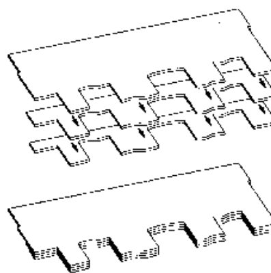
Figure 14-2: Presidential TL Tri-Laminate Construction.
