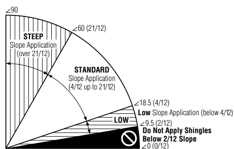
Figure 14-4: Slope definitions
