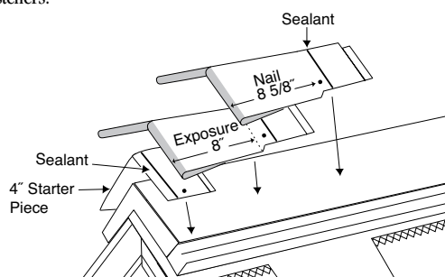
Figure 14-17: Mountain Ridge Hip and ridge application.
