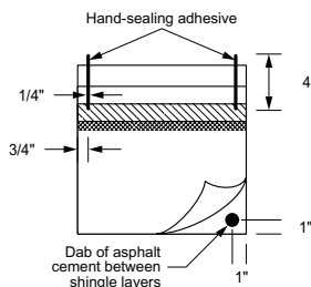
Figure 14-22: Hand seal caps as shown.
