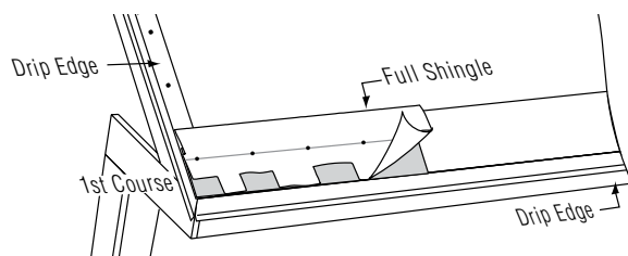
Figure 14-12: First Course.
