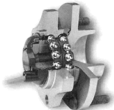
Hub bearing Gen. 3 - ABS/TCS (fig. 3)
