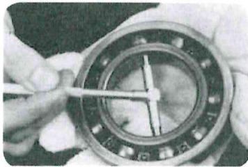
A simple inspection can provide valuable insight into bearing performance and failure. (fig. 1)
