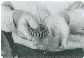
To lubricate the bearing, force grease around the outside of the bearing and between internal parts. (fig. 3)
