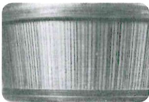
Electric current also causes grooves on the bearing. (fig. 8)
