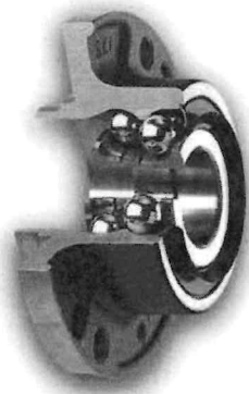
Hub bearing Gen. 2 - ABS/TCS (fig. 2)
