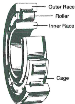
Cylindrical roller bearing
