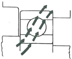
Angular load (fig. 6)
