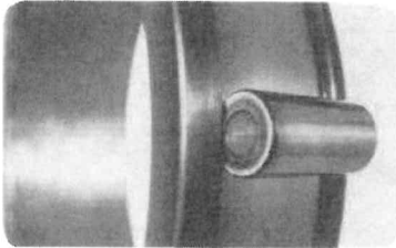
Seizing damage usually appears on the rollers. (fig. 9)
