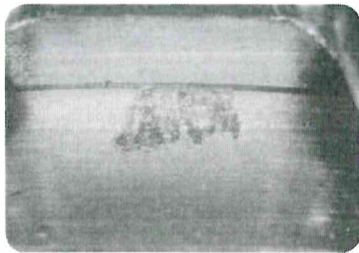
Electric currents passing through a bearing cause arcing and burning. (fig. 7)
