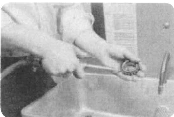
Compressed air may be used to dry the cleaned bearing. (fig. 8)
