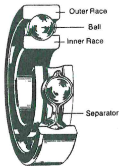
Ball bearing components (fig. 5)
