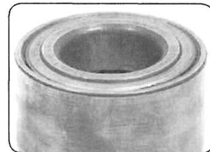
Seal in an oblique position due to wrong fitting during mounting into the knuckle.
