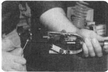
Jaw pullers grip the outer race to remove the bearing. (fig. 2)
