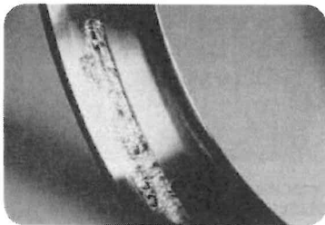
Friction caused by misalignment will discolor the roller path and rollers. (fig. 6)
