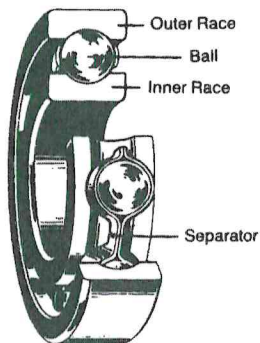
Ball bearing
