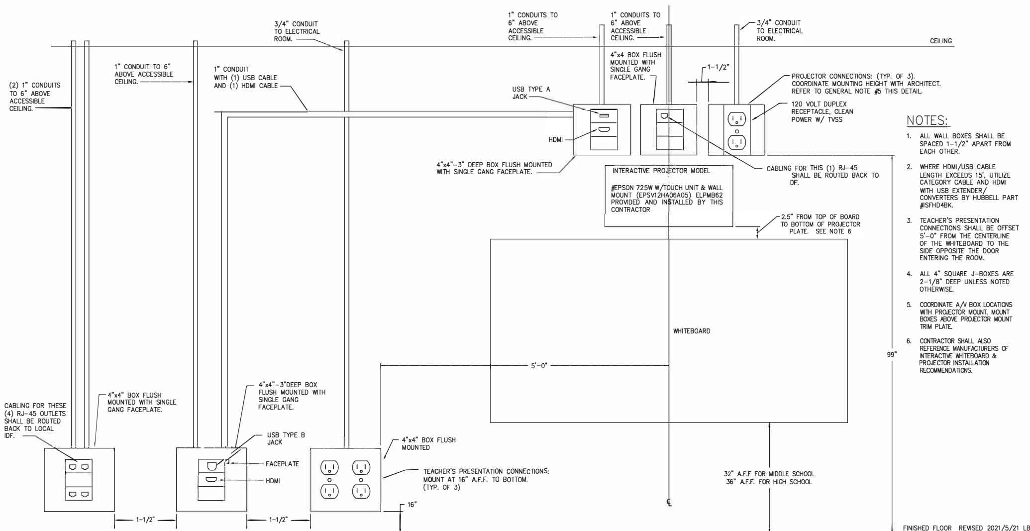
TYPICAL INTERACTIVE PROJECTOR CONDUIT ROUGH-IN DETAIL (MS/HS ONLY).
