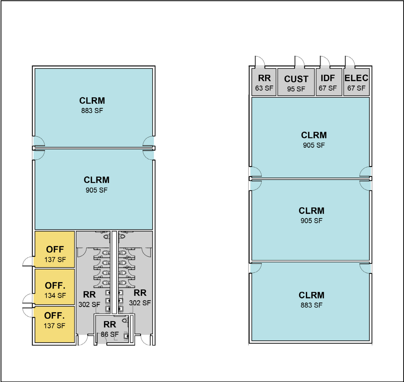
NORTH WING
