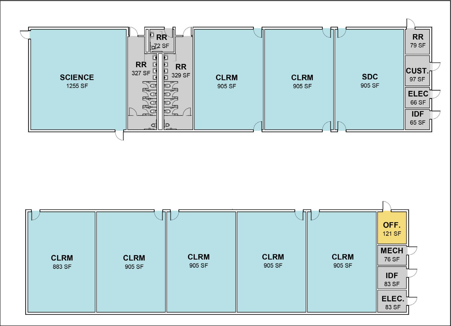
SOUTH WING
