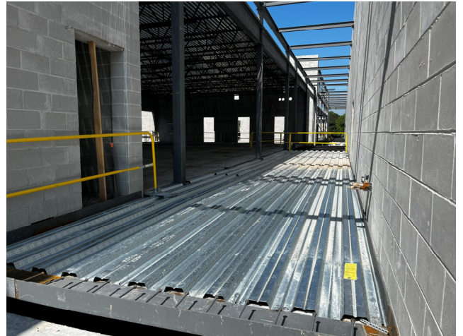
Floor Decking Installed – Area B1
