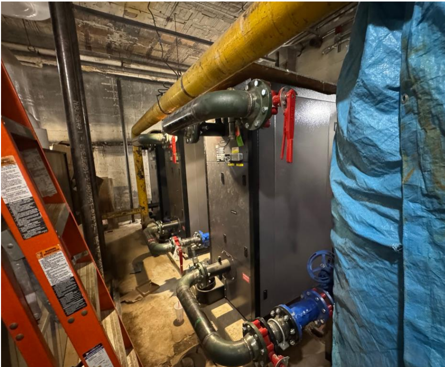
Hempstead ABGS MS – Boiler Room Equipment
