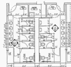
ENLARGED PLAN OF TOILETS 1/4" = 1'-0"
