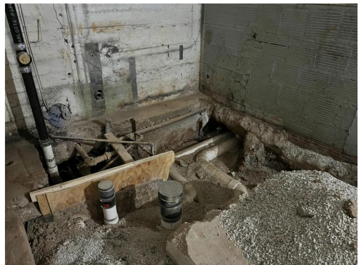
New Under Slab Plumbing – Area A1
