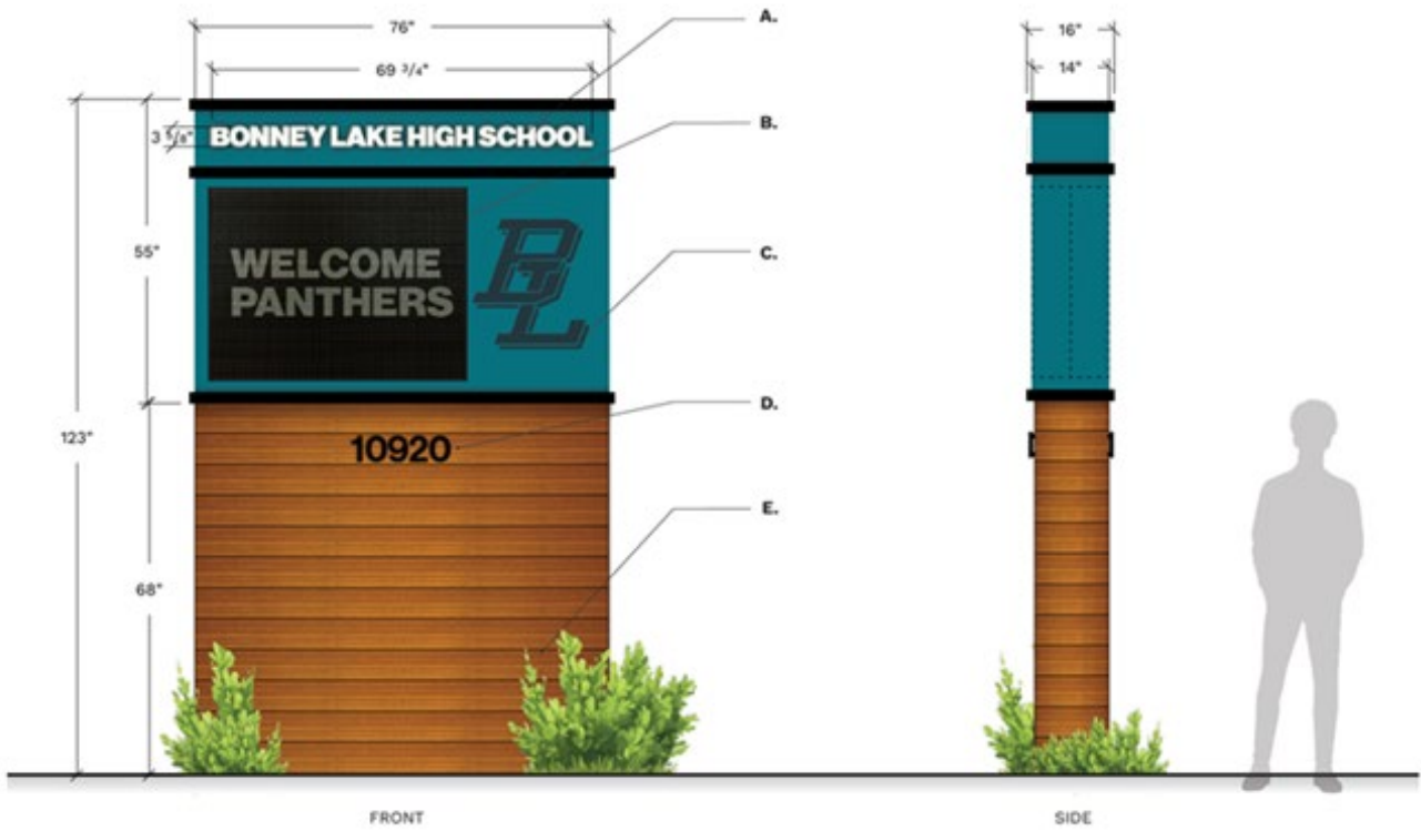
EGD 01 DOUBLE SIDED SCHOOL MONUMENT 1/2" = 1'-0"
