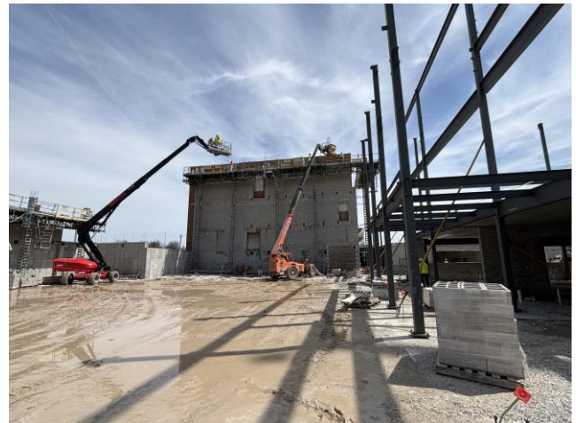
One-Sided Masonry Wall – Area A2
