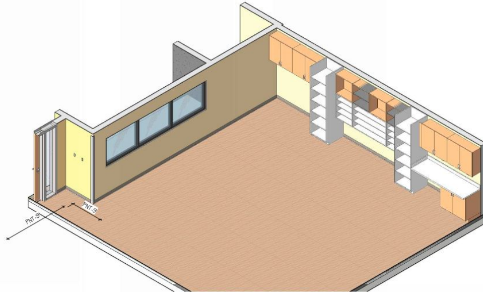
3&4YO CLASS - MILLWORK WALL AXON
