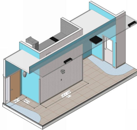
1YO - CORRIDOR TRANSITION AXON
