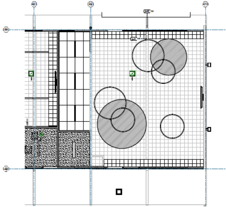
1 ENLARGED RCP - ROOM 10 - LIBRARY 1/8" = 1'-0"
