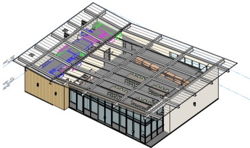
4 BLDG H - 3D VIEW 1
