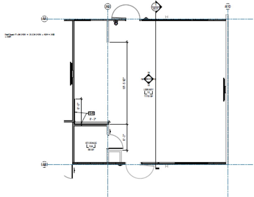
1 ENLARGED FLOOR PLAN - ROOM 10 - LIBRARY 1/8" = 1'-0"
