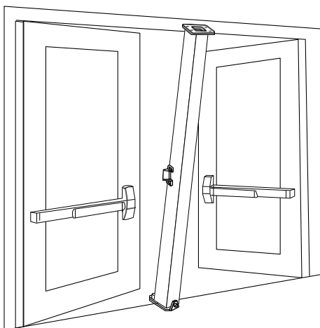
Removable mullions
