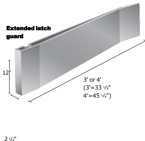
Latch guard
