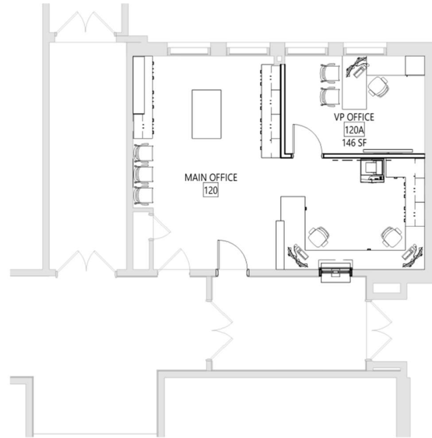
PROPOSED LAYOUT
