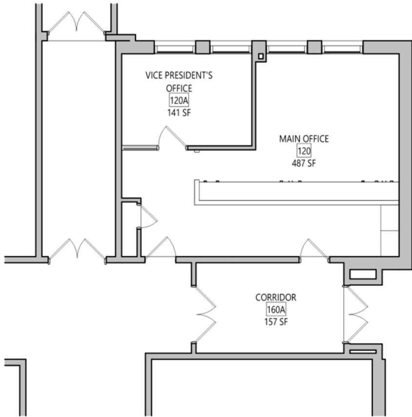
EXISTING LAYOUT
