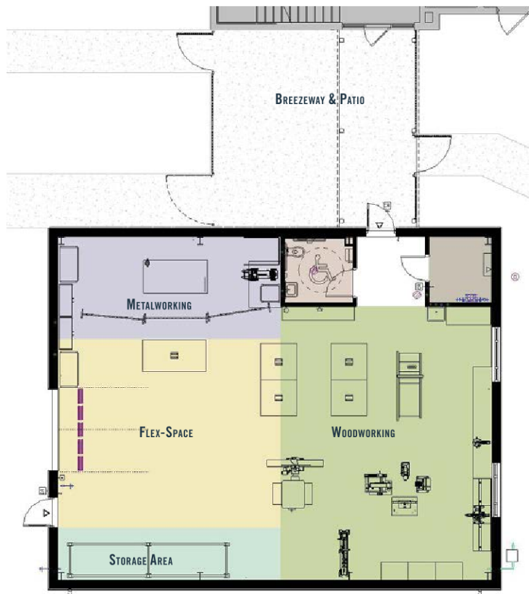
▲ Floor Plan
