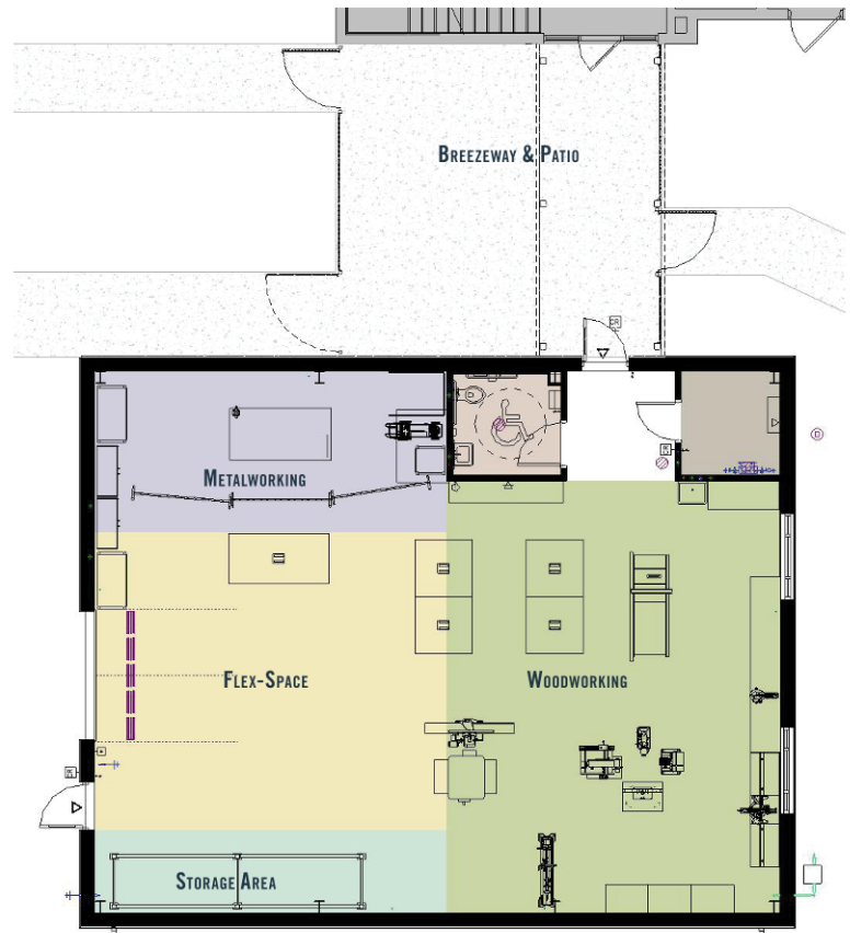
▲ Floor Plan
