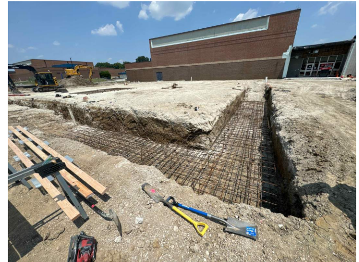
SVMS - Footings
