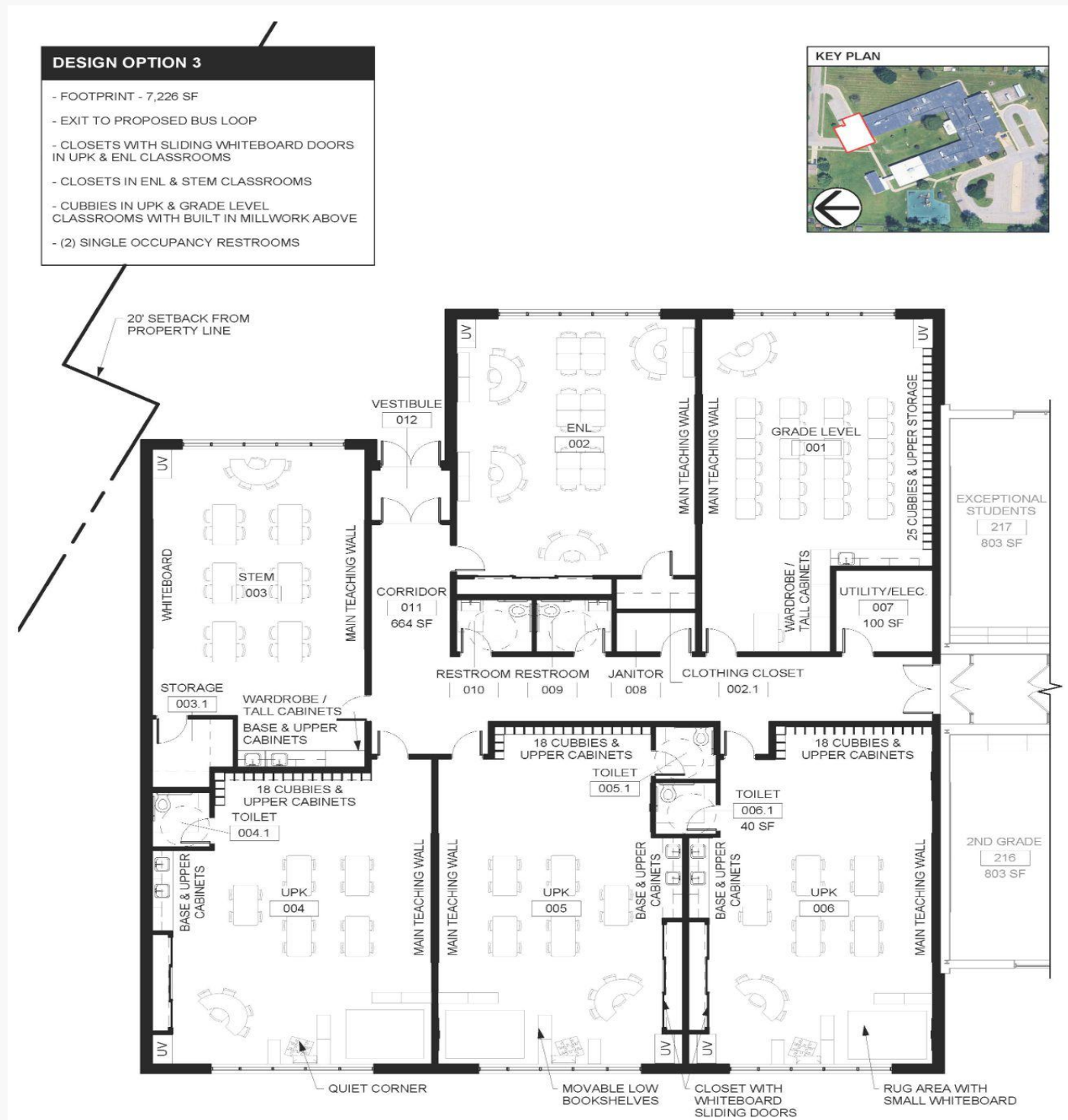
1 ADDITION DESIGN OPTION 3 - FLOOR PLAN SCALE: 1" = 10'-0"
