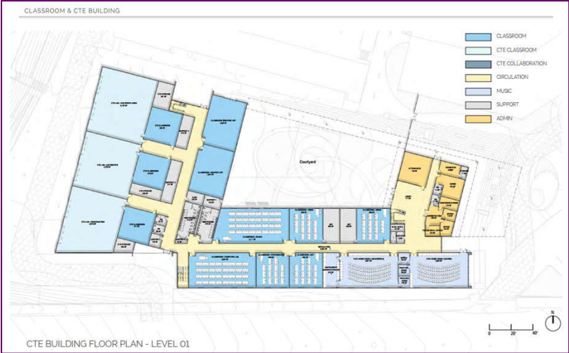
CTE Building Floor Plan (Level 01)
