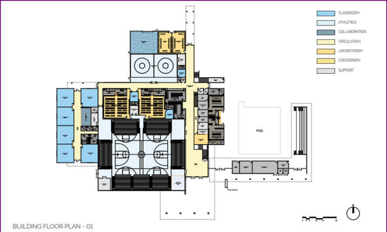
Athletic Center - Building Floor Plan 01
