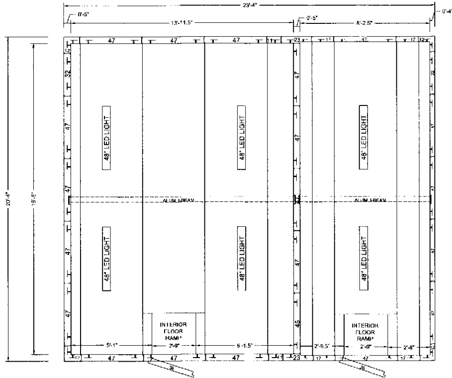
FREEZER WITH FLOOR
