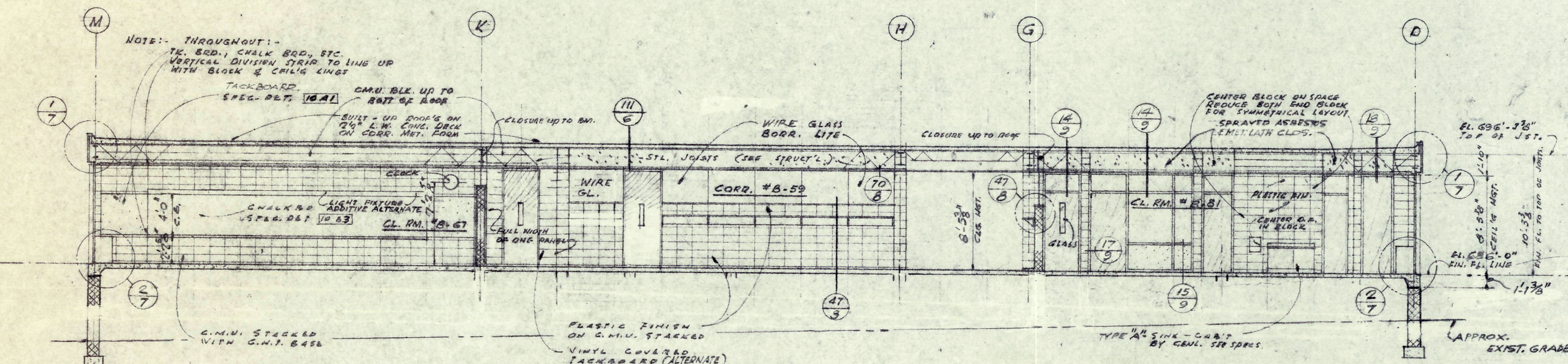
SECTION "Z-6"
