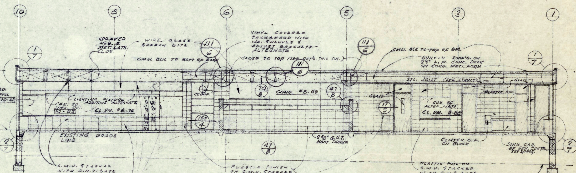
SECTION - "AL-6"
