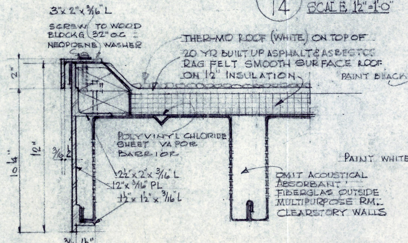
RAKE DETAIL SCALE 3/8" = 1'-0"
