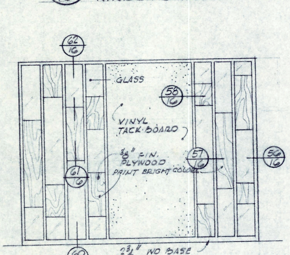
48 COAT RACK @ KINDERGARTENS
