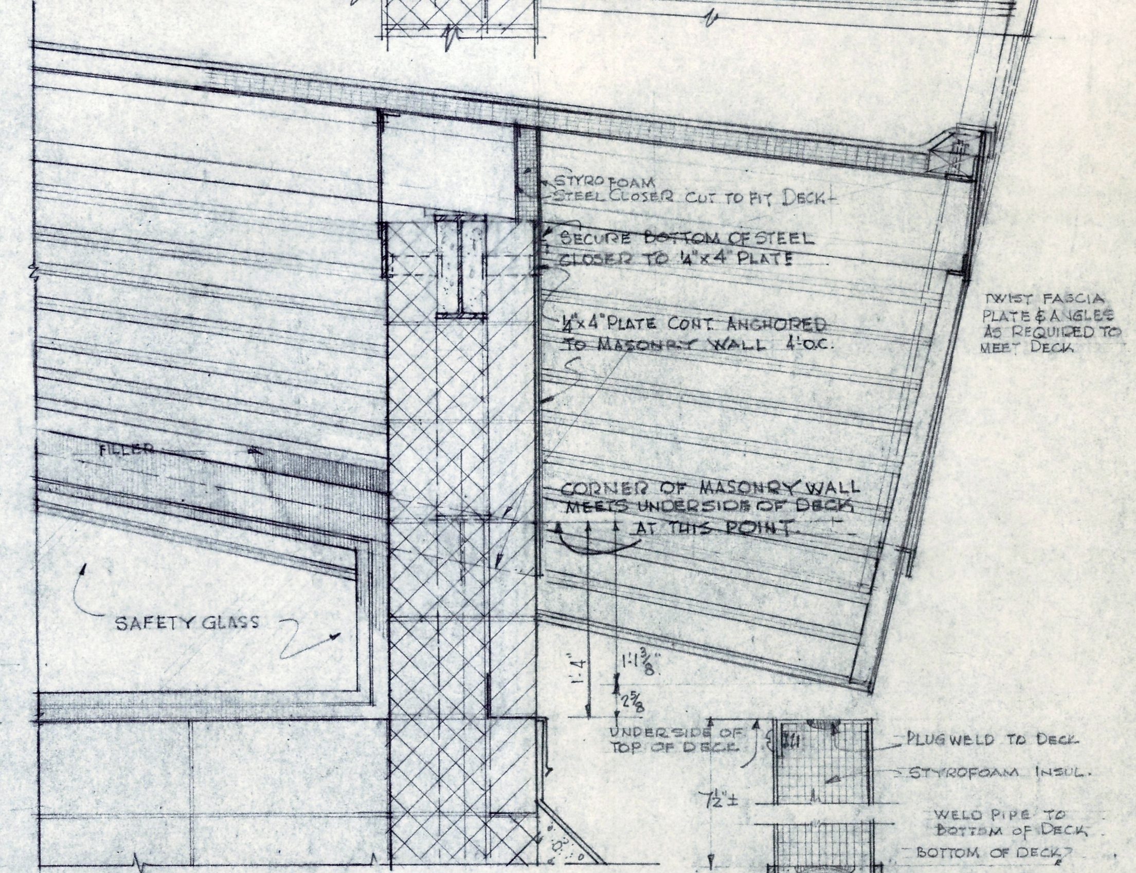
84 SECTION SCALE 1/2" = 1'-0"
