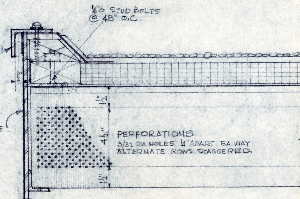
84 SECTION SCALE 1/2" = 1'-0"
