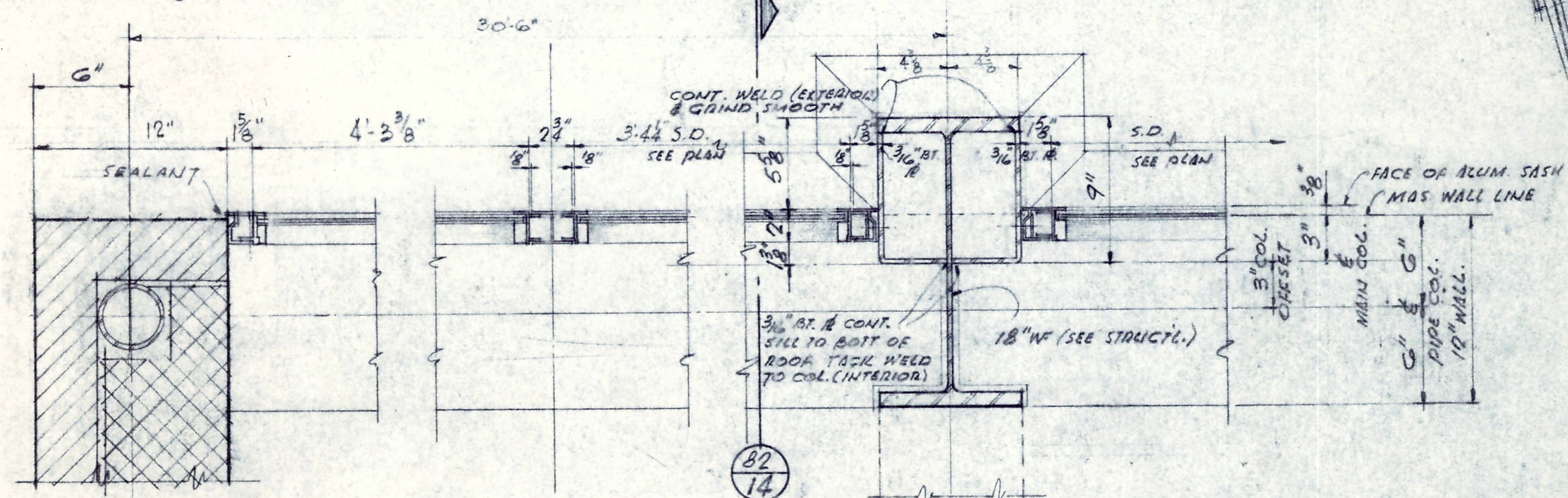
CLERESTORY PLAN - MULTI-PURPOSE RM. SCALE - 3/8" = 1'-0"
