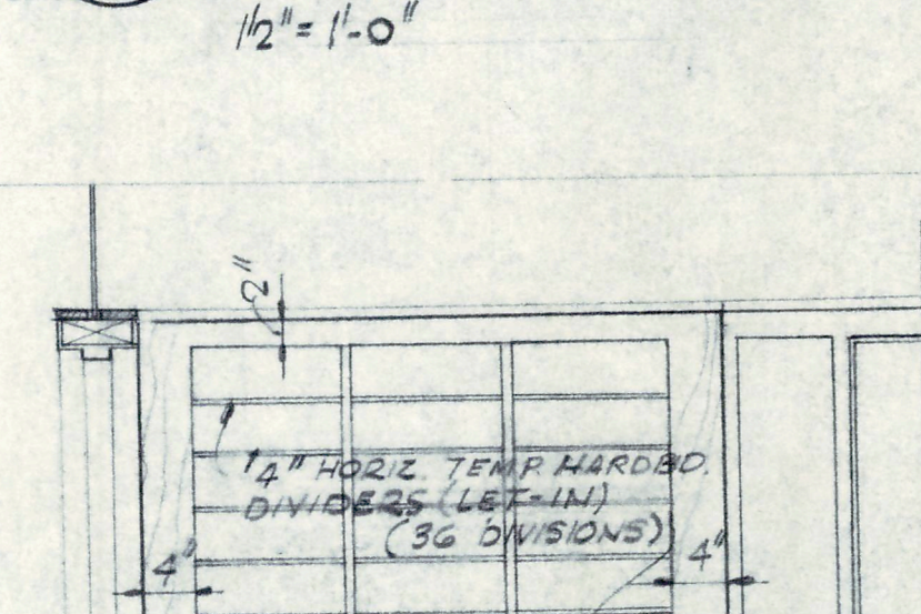
50 COAT RACKS @ COAT RMS. #A-5 & 4-G
