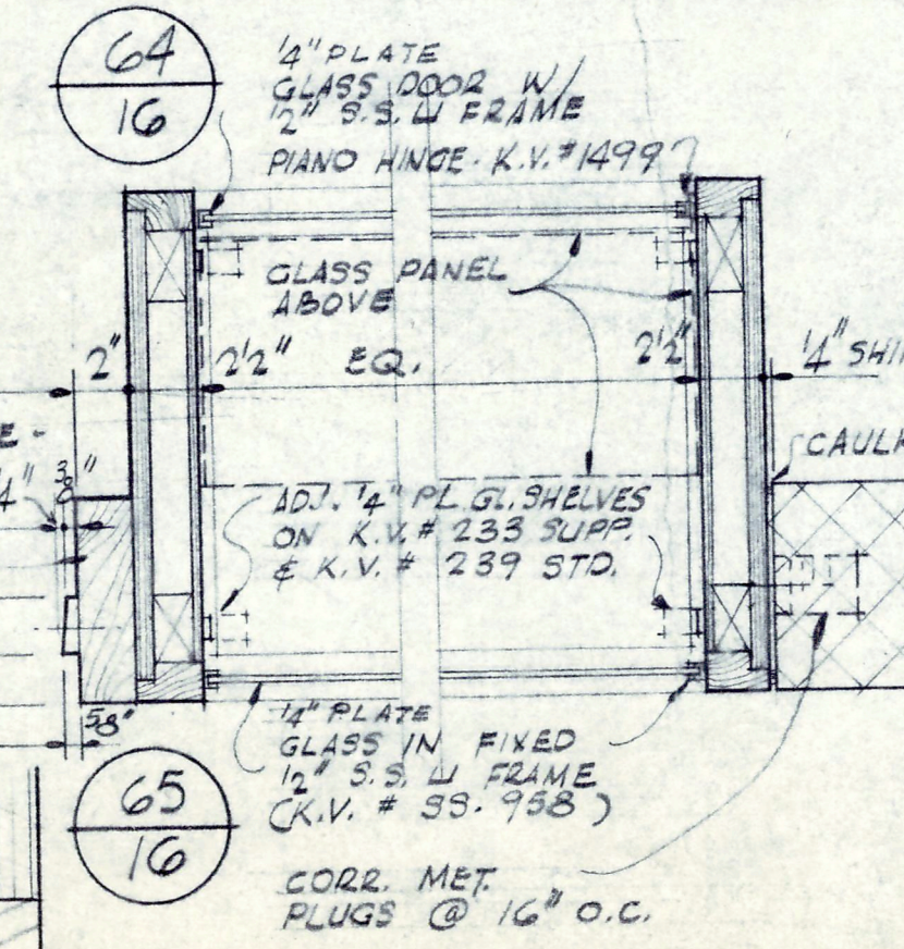
PLAN - DISPLAY CASE
