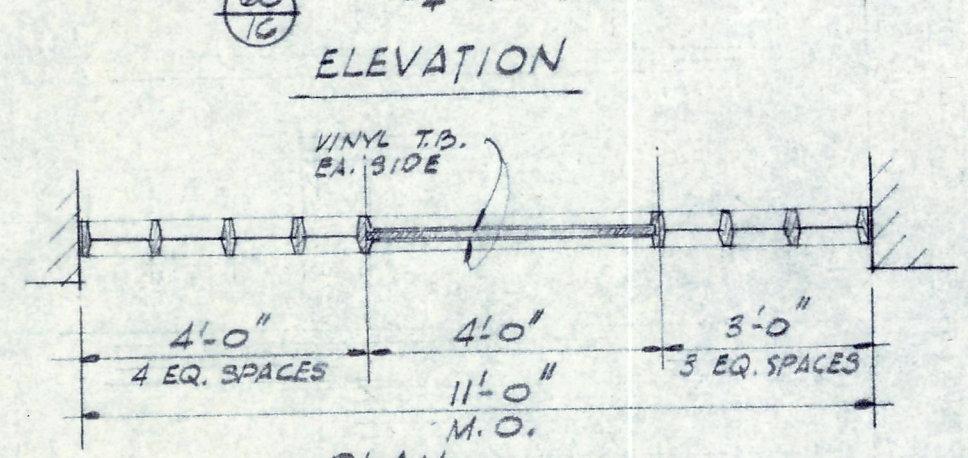
PARTITION - OFFICE #A-20
