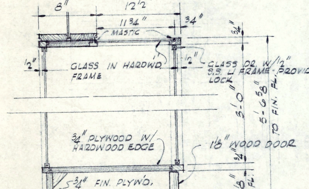
LIBRARY ENTRANCE ELEV. - 36" x 1'-0"
