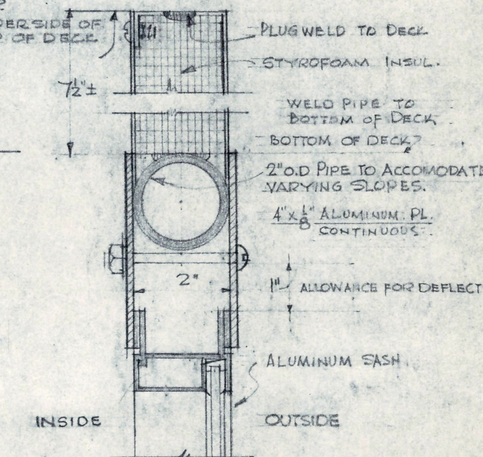
HALF FULLSIZE DETAIL OF SASH CONNECTION TO METAL DECK
