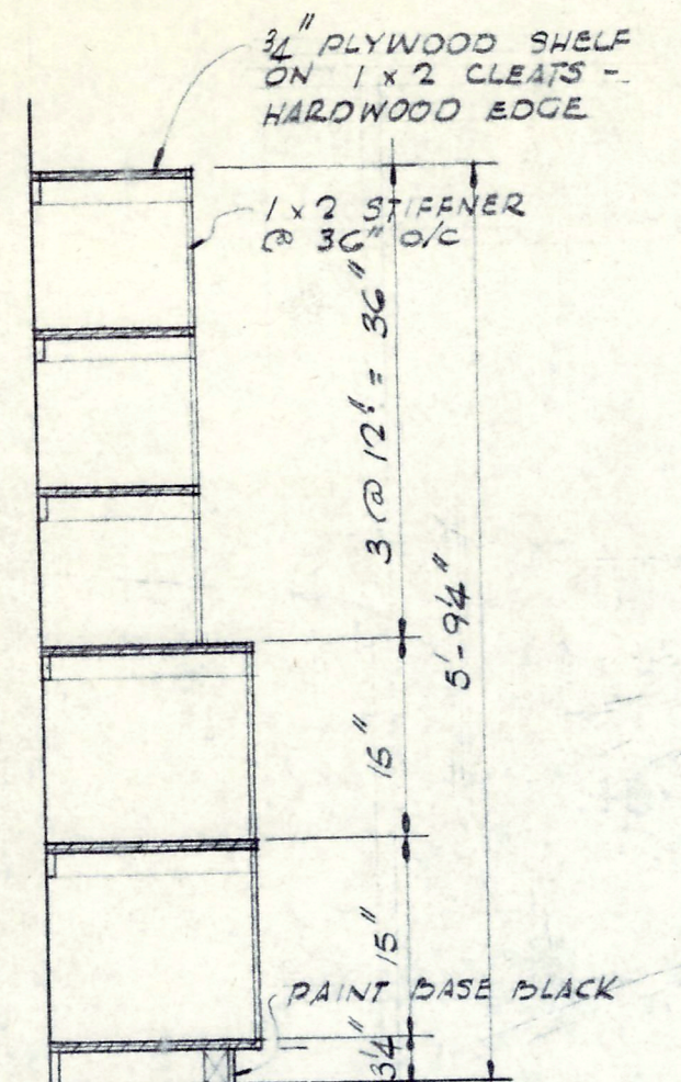
SECTION - CLOSET SHELVING
