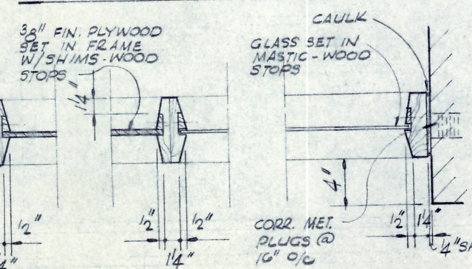
PARTITION - OFFICE #A-20
