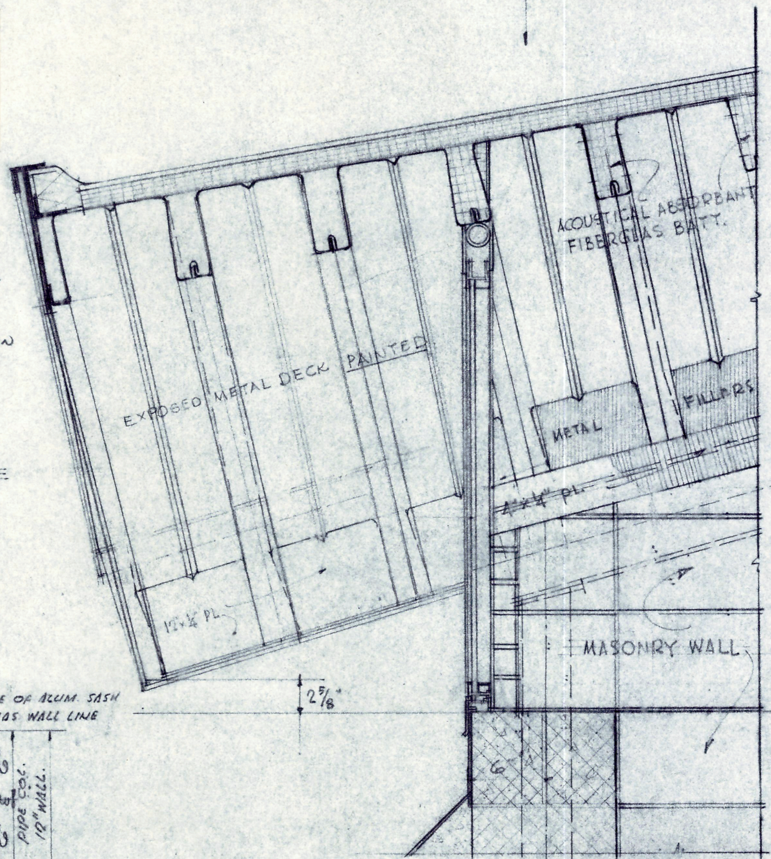
83 SECTION SCALE 1/2" = 1'-0"
