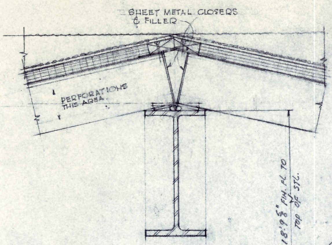
86 DETAIL SECTION NORTH & SOUTH RIDGE SCALE 1/2" = 1'-0"
