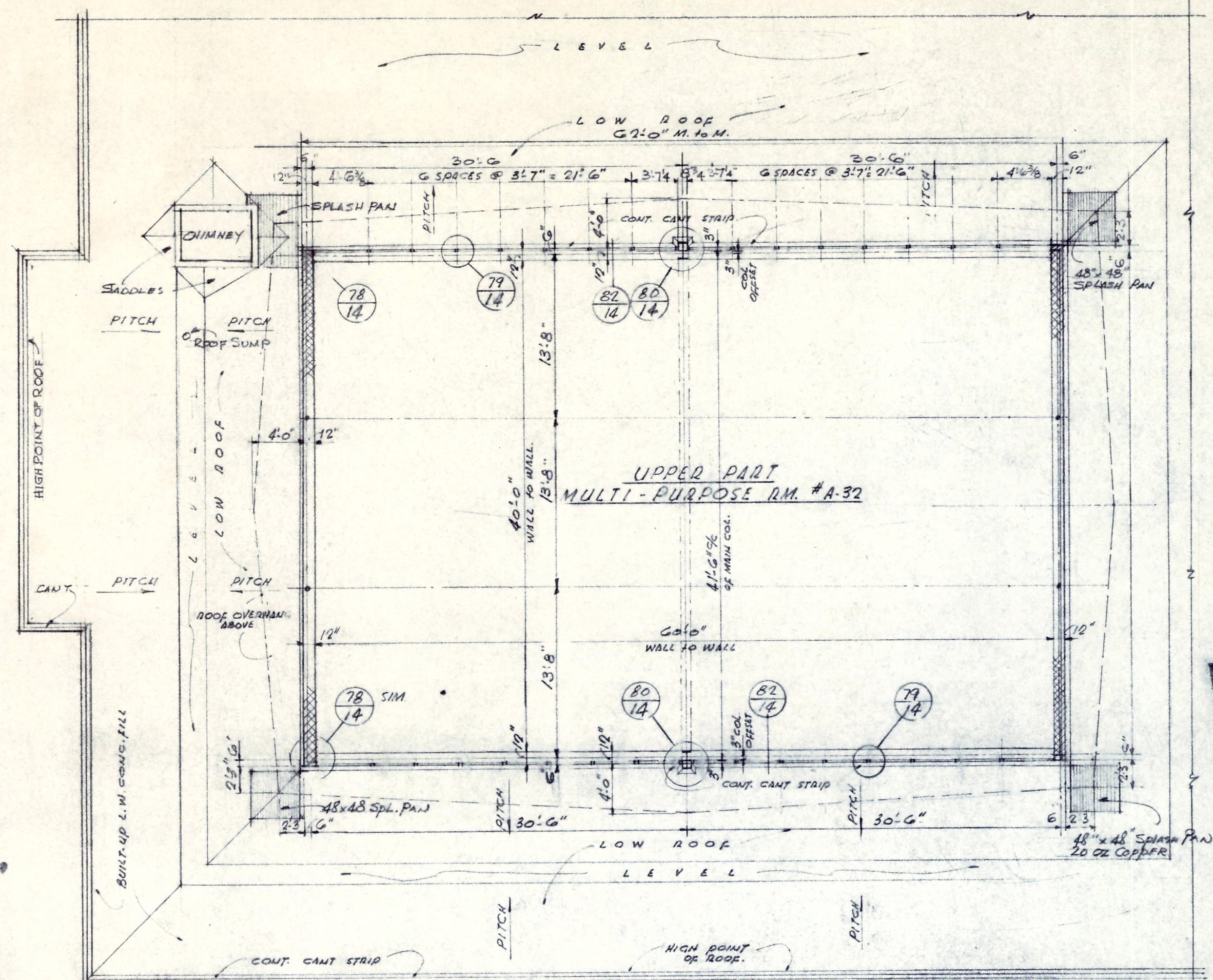
CLERESTORY PLAN - MULTI-PURPOSE RM. SCALE - 3/8" = 1'-0"
