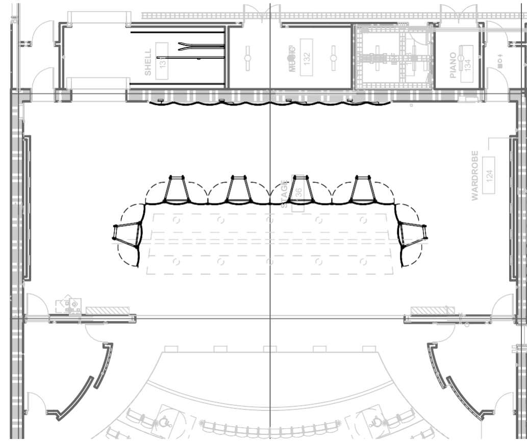
2 ORCHESTRA SHELL TOWER - CONFIG #2 1/16" = 1'-0"
