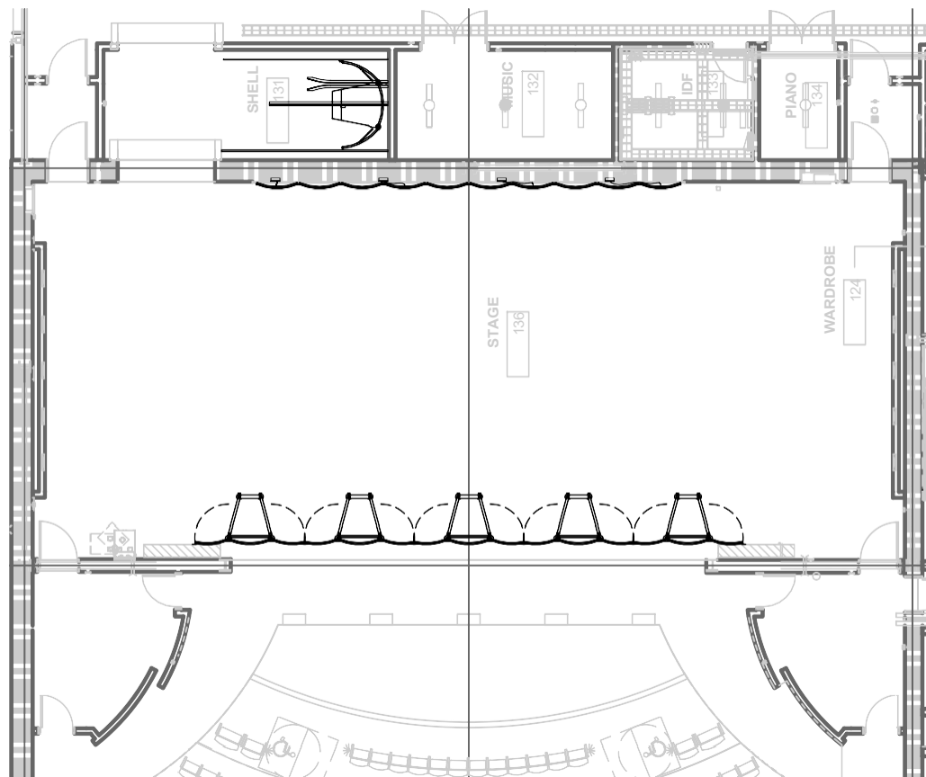
3 ORCHESTRA SHELL TOWER - CONFIG #3 1/16" = 1'-0"
