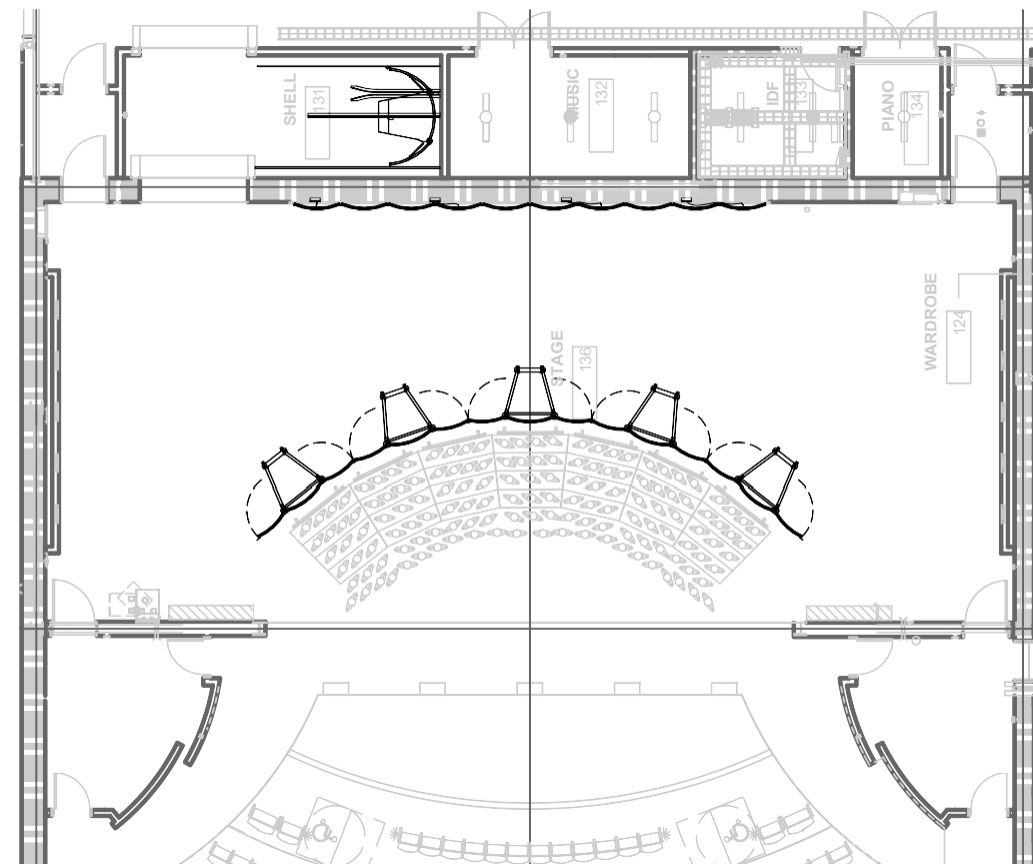
4 ORCHESTRA SHELL TOWER - CONFIG #4 1/16" = 1'-0"
