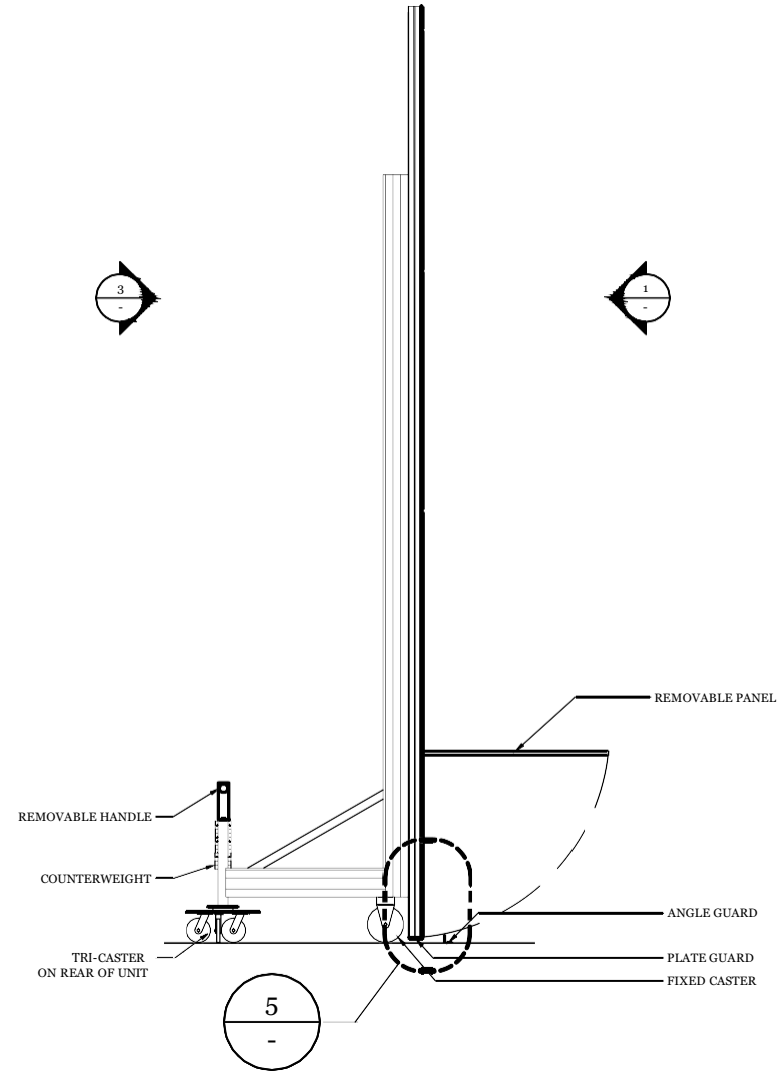
2 ORCHESTRA SHELL TOWER DETAIL SECTION 1/4" = 1'-0"
