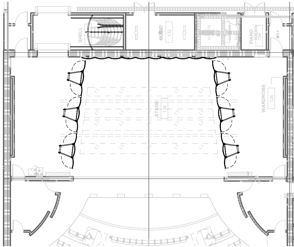
1 ORCHESTRA SHELL TOWER - CONFIG #1 1/16" = 1'-0"
