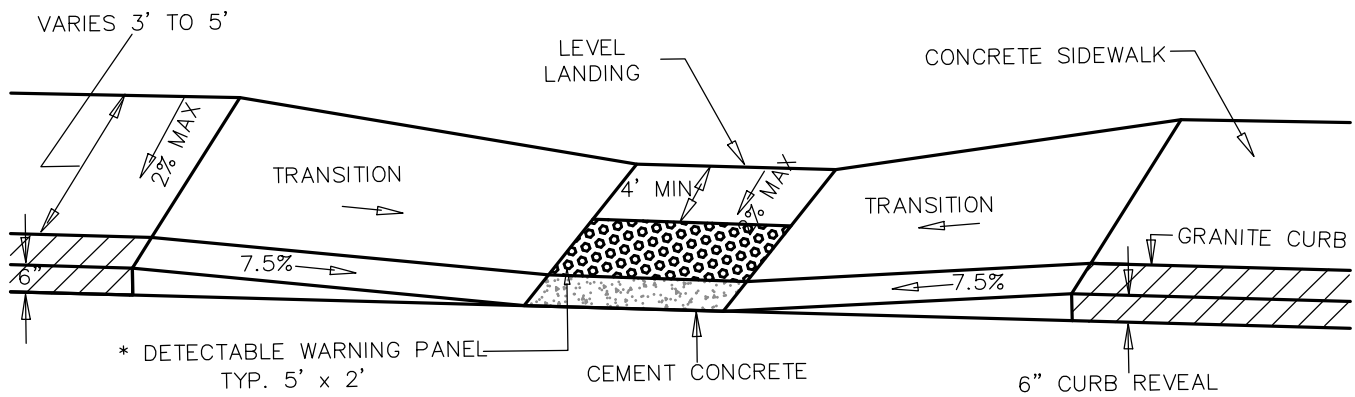
WHEELCHAIR RAMP NARROW SIDEWALK PLAN
