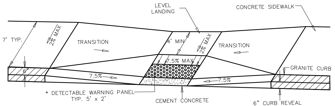
WHEELCHAIR RAMP TYPICAL SIDEWALK PLAN
