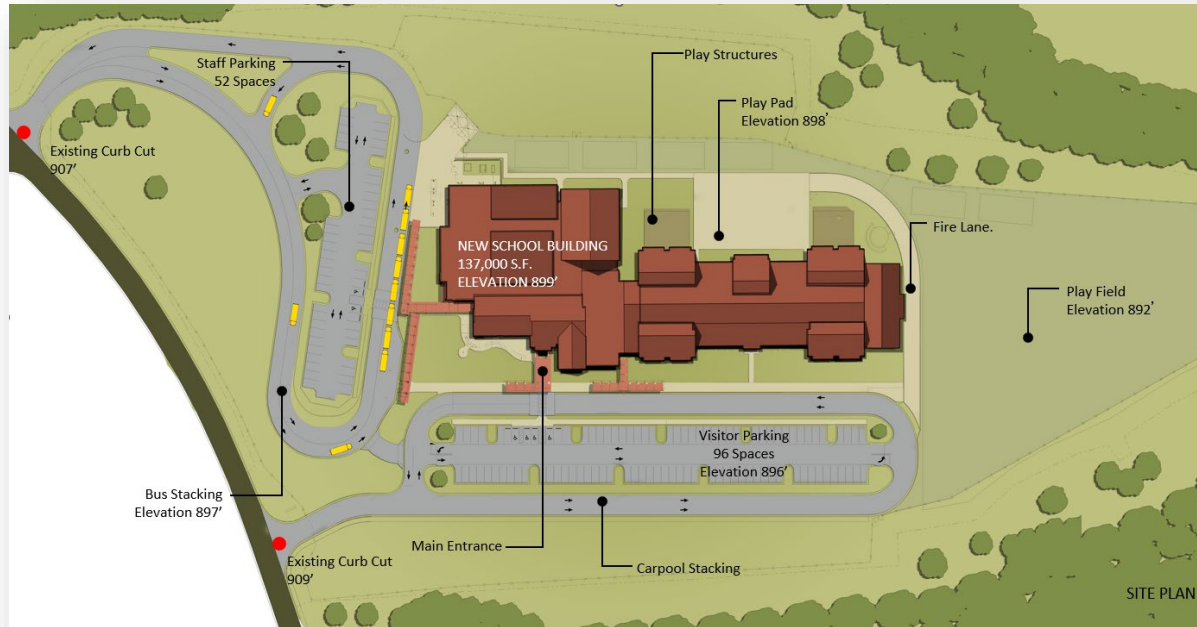
SITE PLAN
