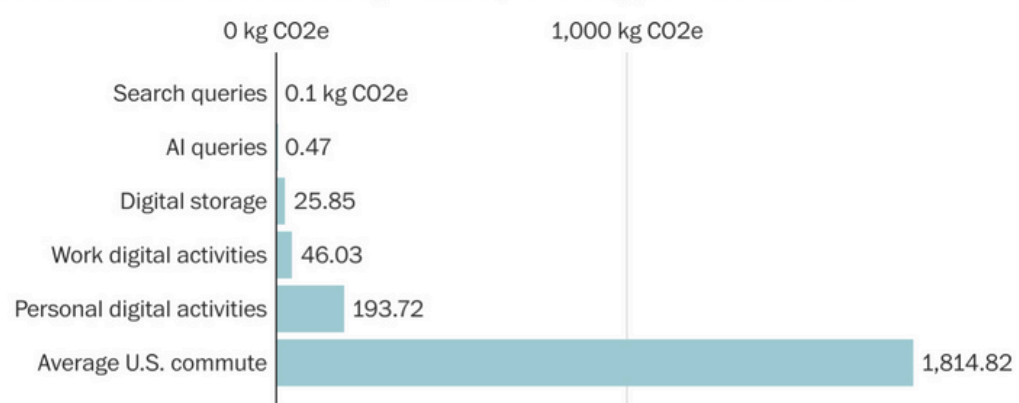
Annual GHG emissions by activity for a typical American
