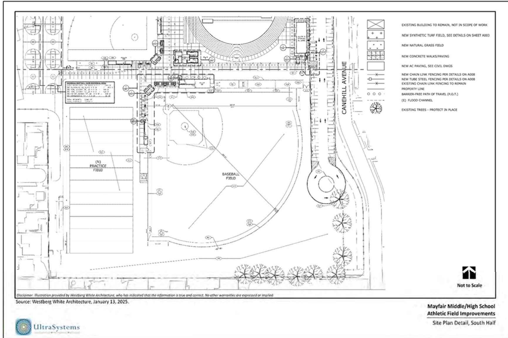
Figure 3.3-3 SPORTS FIELD IMPROVEMENT PROJECT SITE PLAN (ENLARGED SOUTH END)
