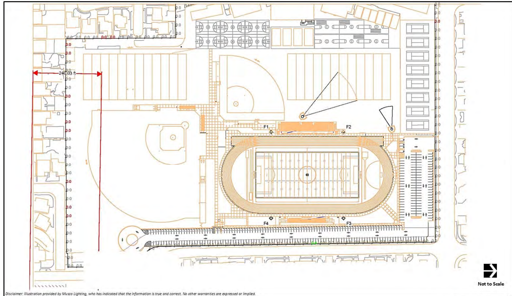
Figure 4.1-4 CONSTANT ILLUMINATION – HORIZONTAL FOOTCANDLES
