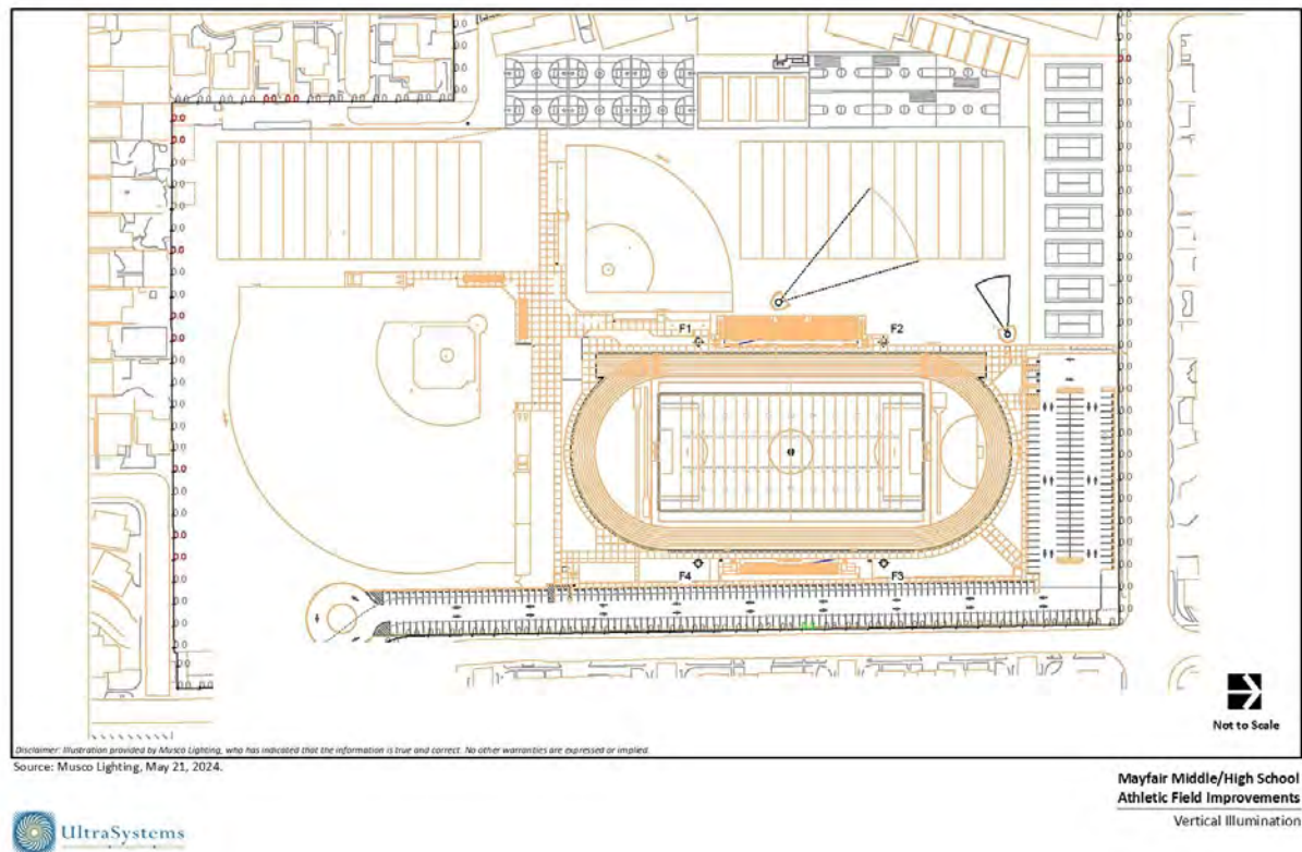
Figure 4.1-3 CONSTANT ILLUMINATION – VERTICAL FOOTCANDLES
