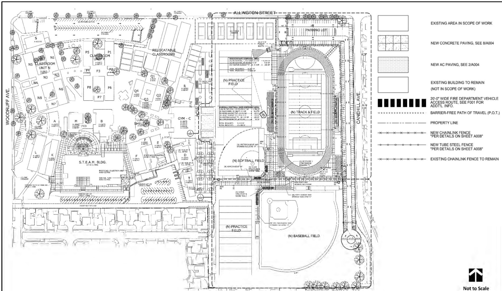
Figure 3.3-1 SPORTS FIELD IMPROVEMENT PROJECT SITE PLAN
