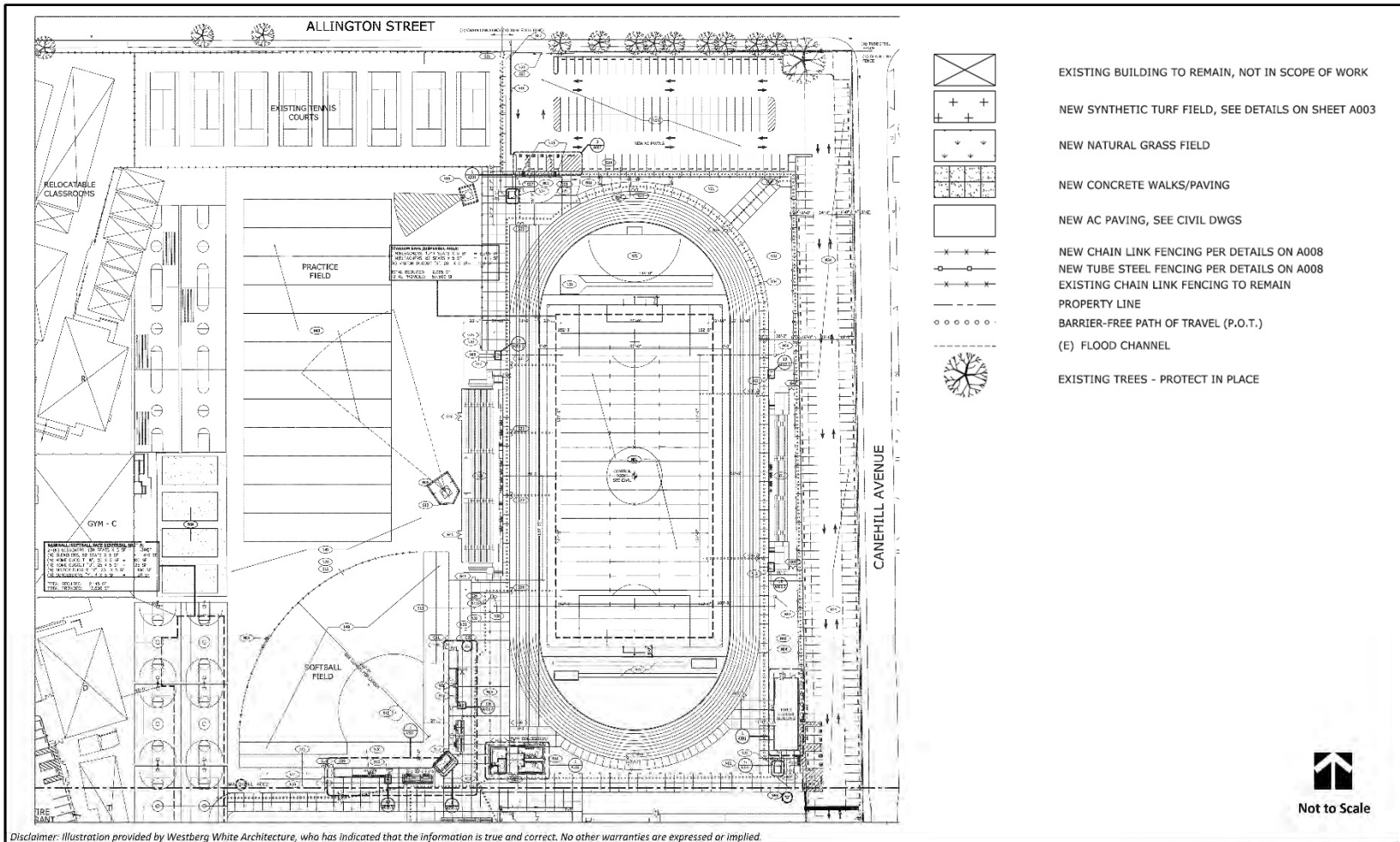
Figure 3.3-2 SPORTS FIELDS IMPROVEMENT PROJECT SITE PLAN (ENLARGED NORTH END)
