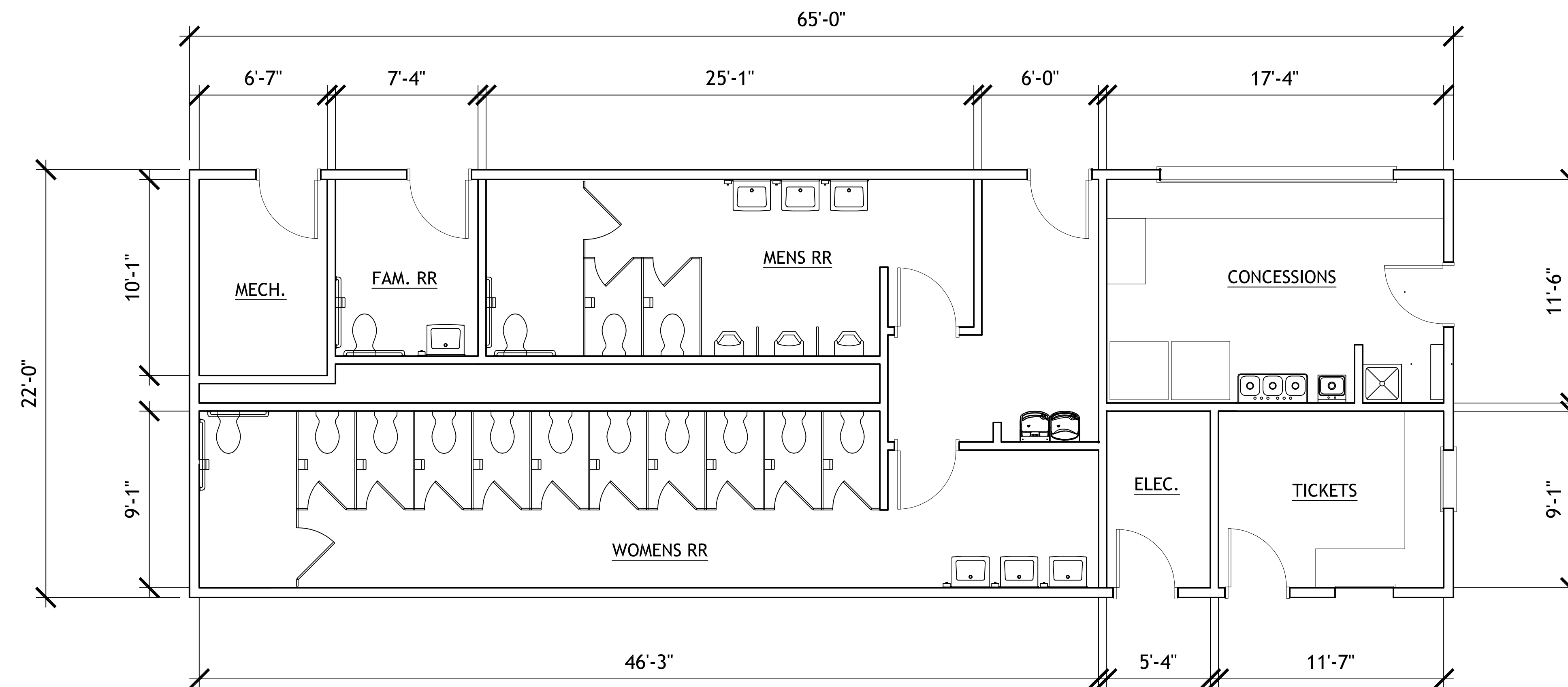
PROPOSED RESTROOM AND CONCESSIONS BUILDING
