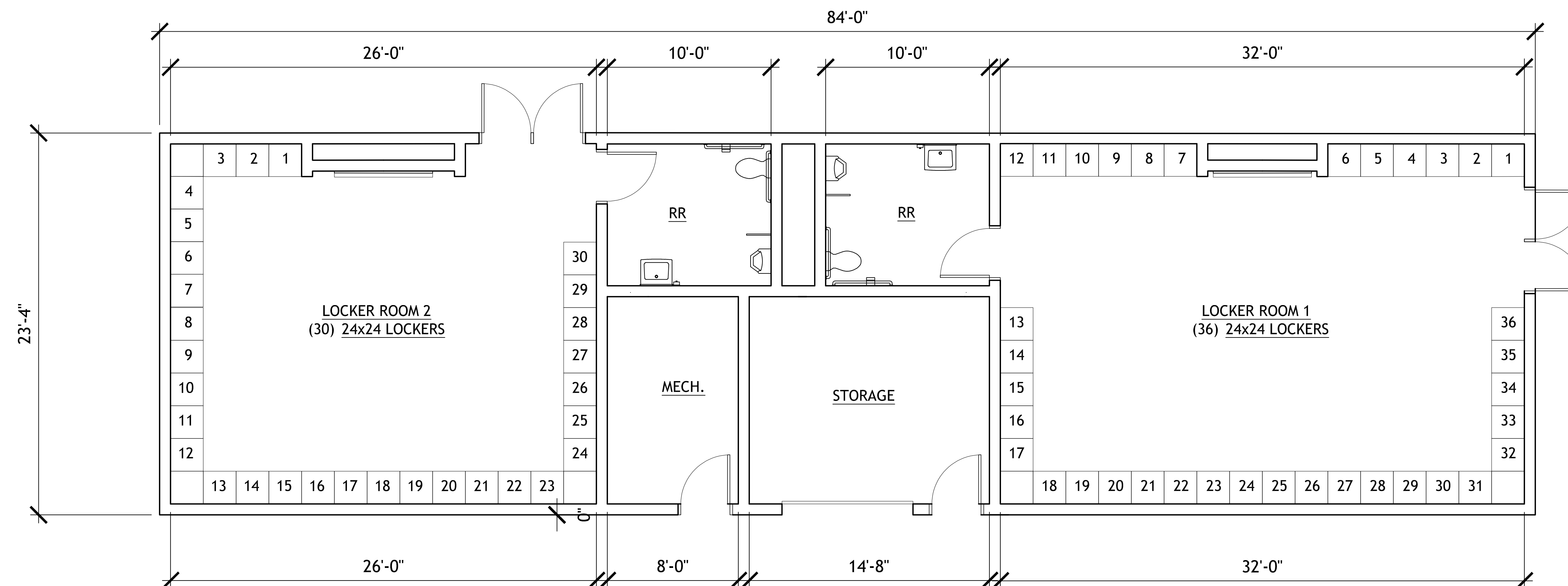
PROPOSED LOCKER ROOM BUILDING
