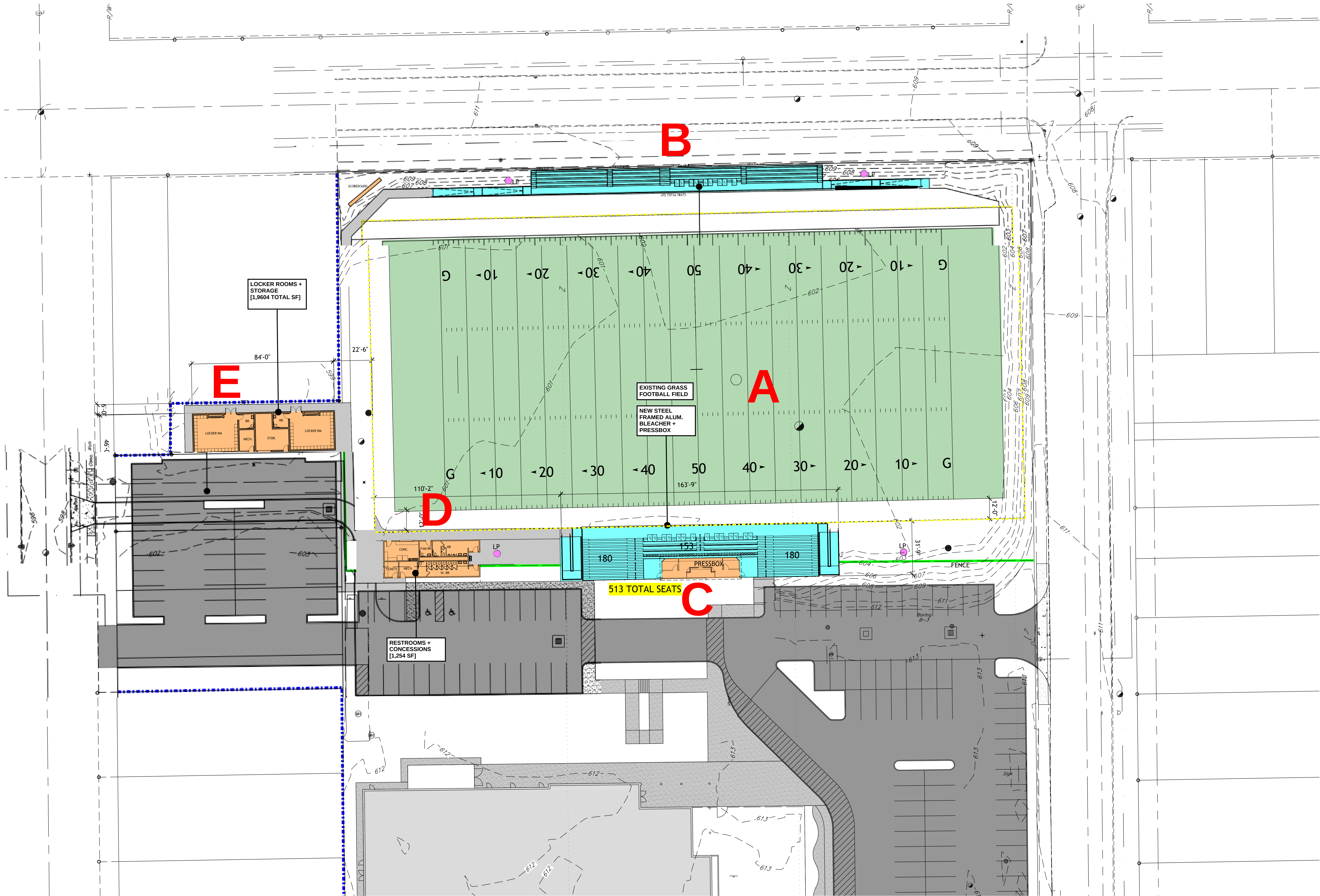
OPTION 3 - NEW BLEACHER WITH PRESSBOX AND RR/CONCESSION BUILDING AND LOCKER ROOM BUILDING
