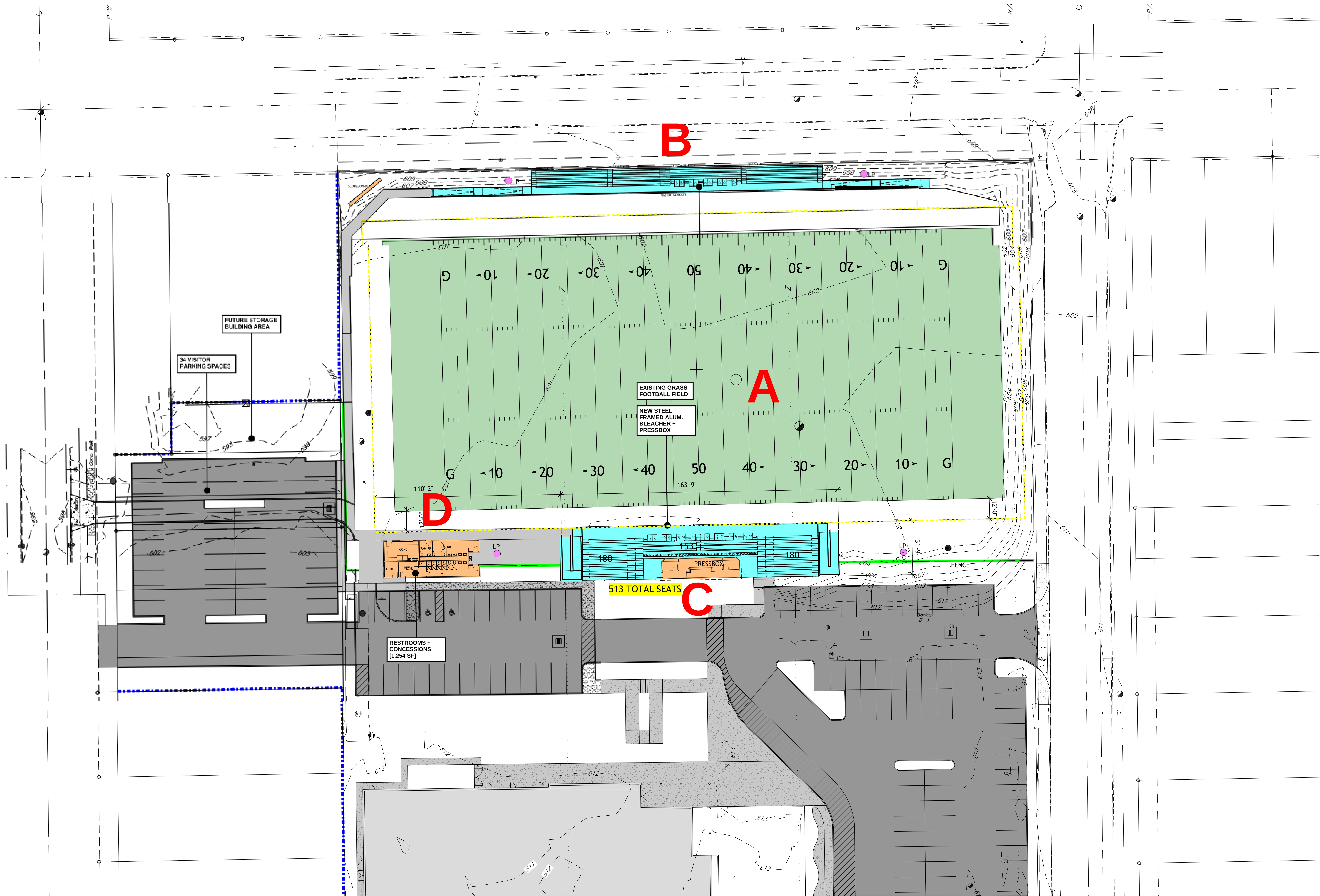
OPTION 2 - NEW BLEACHER WITH PRESSBOX AND RR/CONCESSION BUILDING
