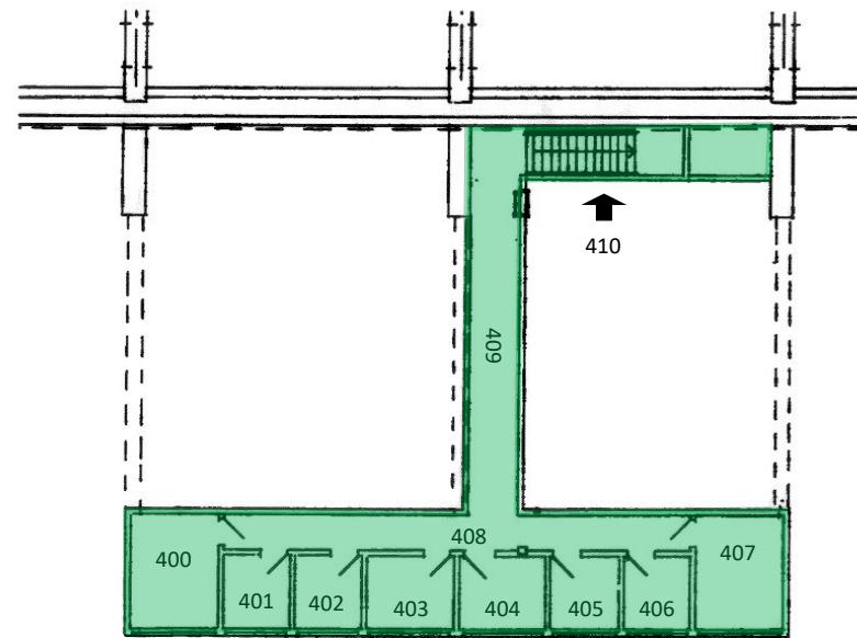
EXISTING GRANDSTAND - PRESSBOX LEVEL SCALE: 1/8" = 1'-0"
