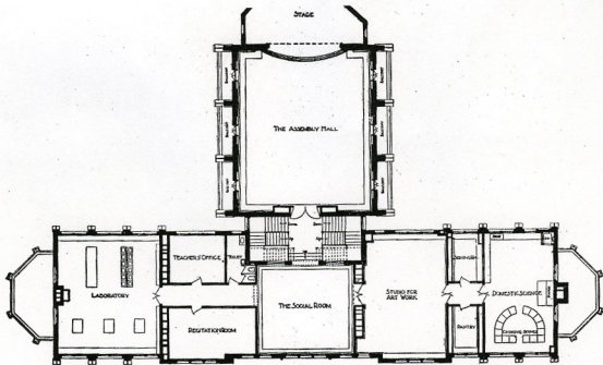
PLANS OF THE NEW SEMINARY BUILDING: SECOND FLOOR, WITH ASSEMBLY HALL.
