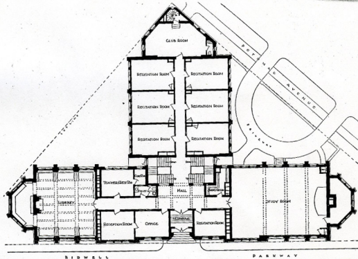
PLANS OF THE NEW SEMINARY BUILDING: FIRST FLOOR, WITH RECITATION ROOMS.
