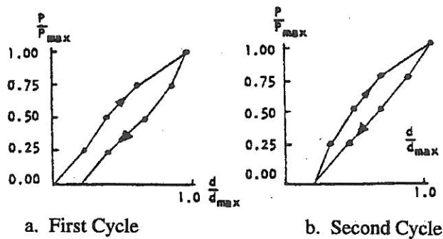
Figure 1. Static Load Test Load-Deflection Curves
