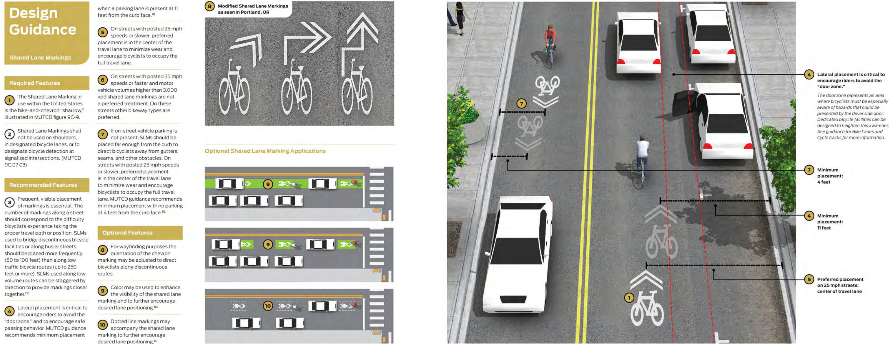
Figure 2.13 Shared Lane Marking Design Guidance, NACTO
