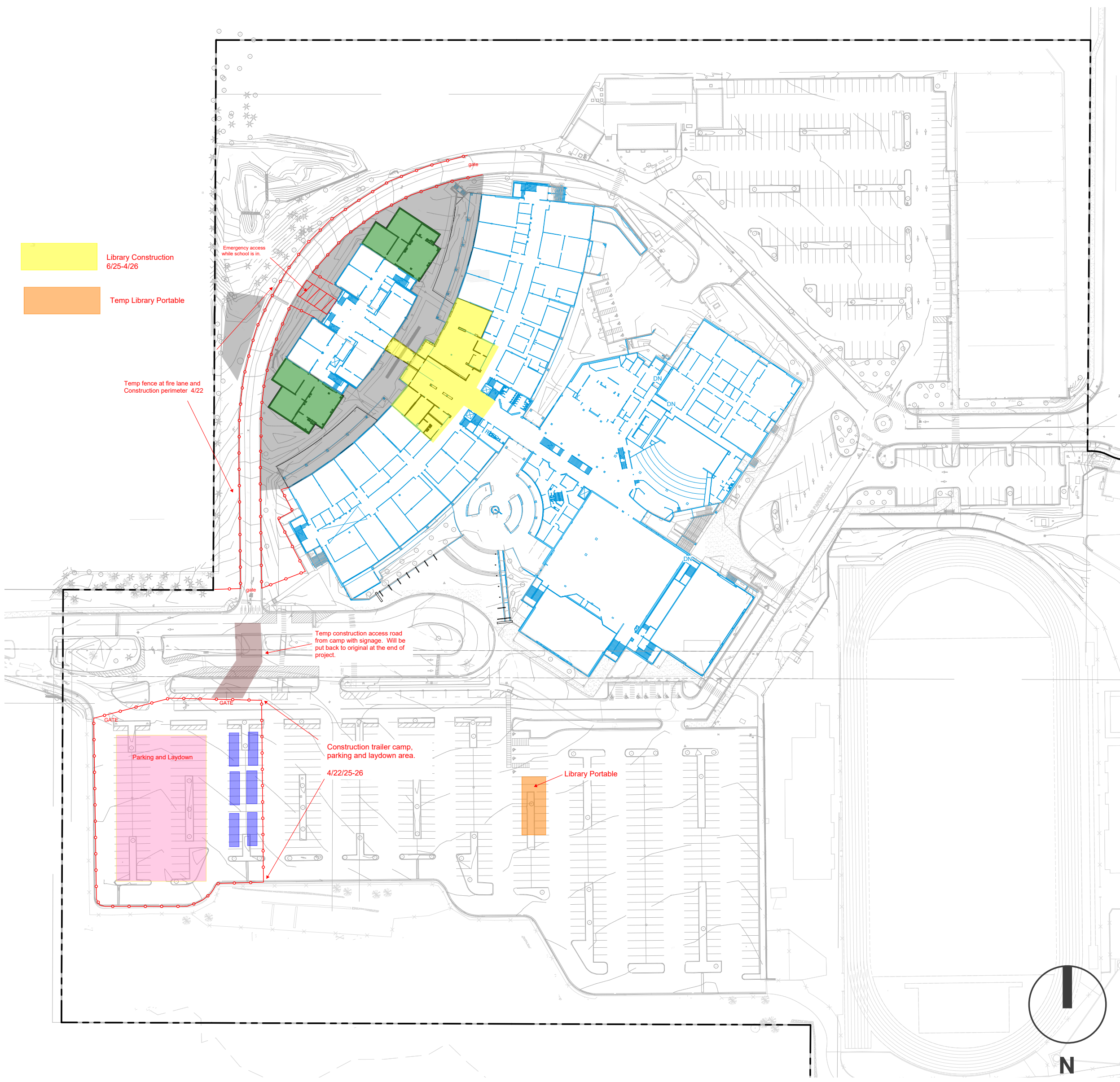
CONSTRUCTION PHASING PLAN 2025 - 2026 SCHOOL YEAR
