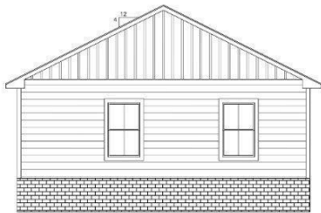
2 A-2 LEFT ELEVATION SCALE 1/4" = 1'-0"
