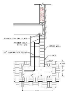
1 FOOTING DETAILS SCALE 1/4" = 1'-0"
