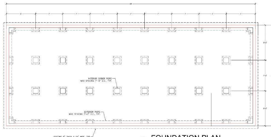
2 FOUNDATION PLAN SCALE 1/4" = 1'-0"
