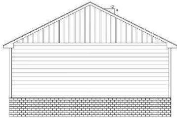
1 A-2 RIGHT ELEVATION SCALE 1/4" = 1'-0"
