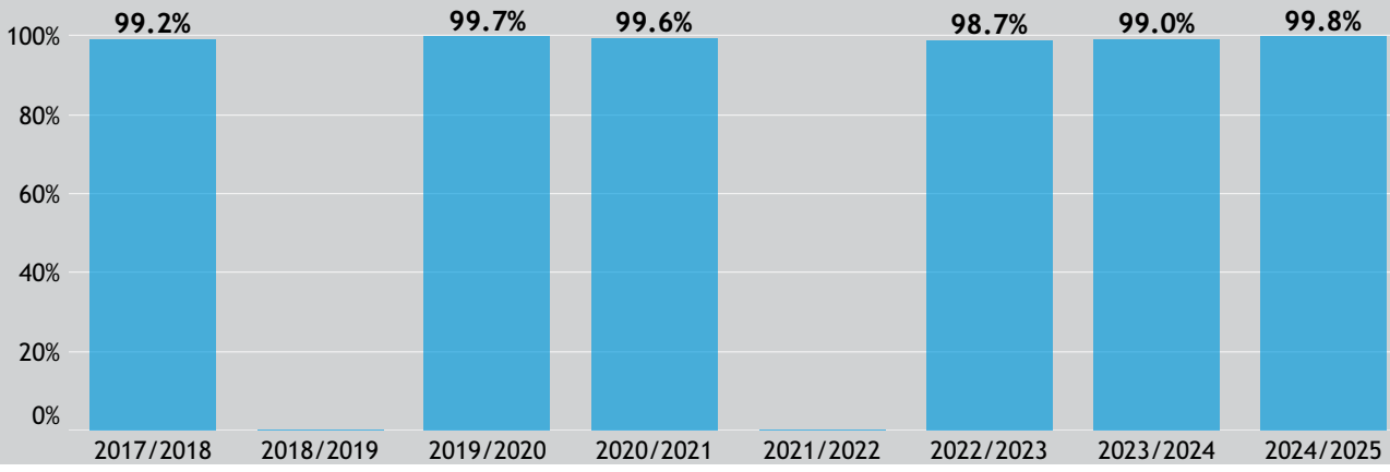
Compliance Rate
