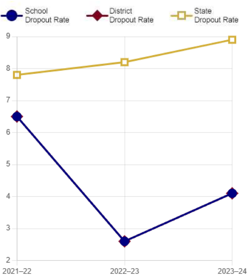
Dropout Rates
