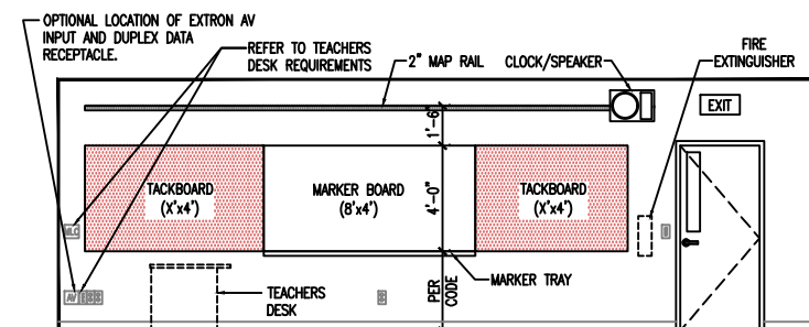
ELEVATION B - SECONDARY (SUPPLEMENTAL) TEACHING WALL
