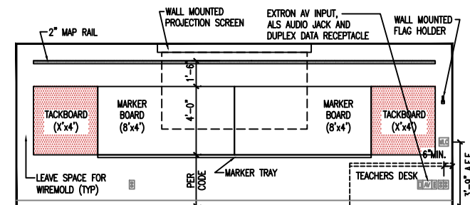
ELEVATION A - PRIMARY (PROJECTION) TEACHING WALL
