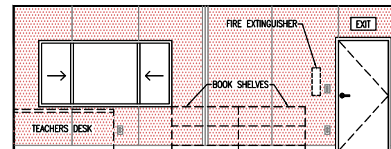
ELEVATION B – ENTRY WALL
