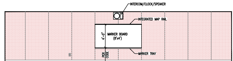
ELEVATION C – SECONDARY (SUPPLEMENTAL) TEACHING WALL
