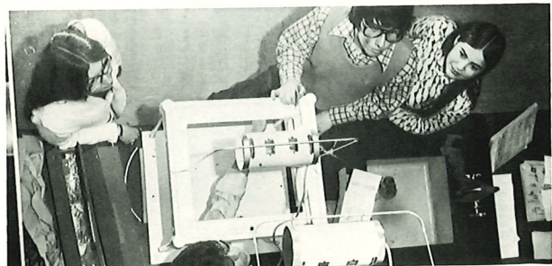
Happiness is the Ripple Tank.
