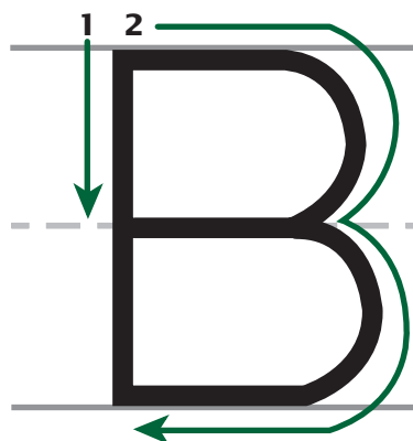
Figure 2. Handwriting-practice diagram
